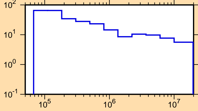
\Delta\sigma/\sigma vs. E for ^{212}\text{Bi}(n,\text{nonel.})
