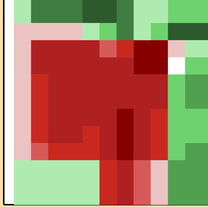
\Delta\sigma/\sigma vs. E for ^{212}\text{Bi}(n,n\text{cont.})
