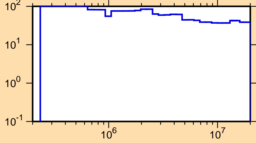
\Delta\sigma/\sigma vs. E for ^{213}\text{Bi}(n,n_1)
