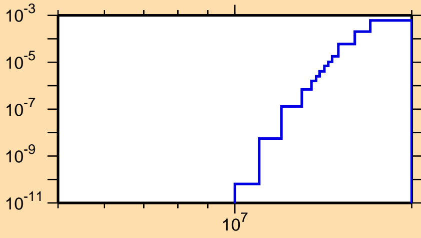
\sigma vs. E for ^{213}\text{Bi}(n,nt)
