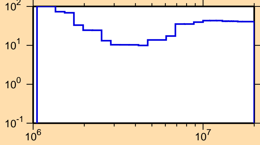
\Delta\sigma/\sigma vs. E for ^{213}\text{Bi}(n,n\text{cont.})
