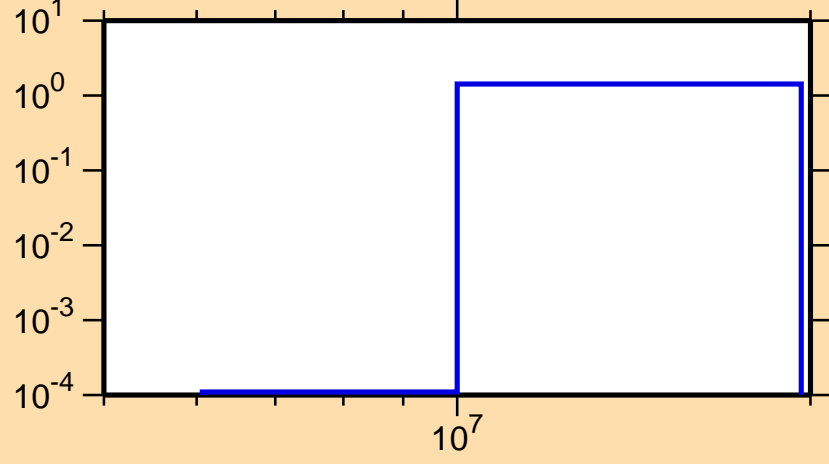
\sigma vs. E for ^{213}\text{Bi}(n,3n)
