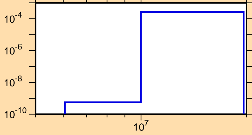
\sigma vs. E for ^{213}\text{Bi}(n,np)
