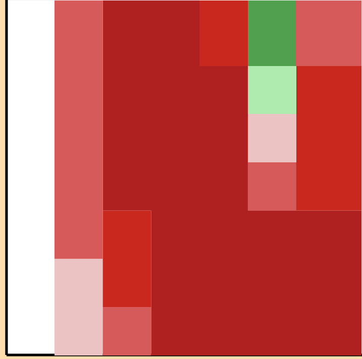
\Delta\sigma/\sigma vs. E for ^{213}\text{Bi}(n,n\text{cont.})
