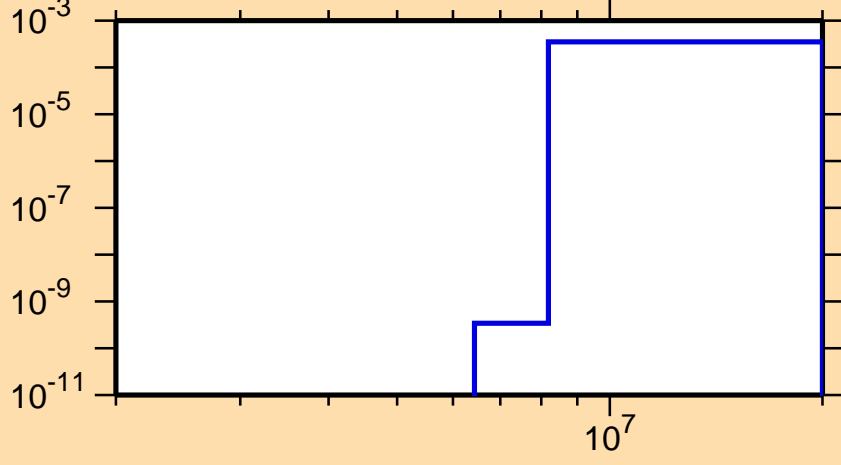
\sigma vs. E for ^{213}\text{Bi}(n,t)
