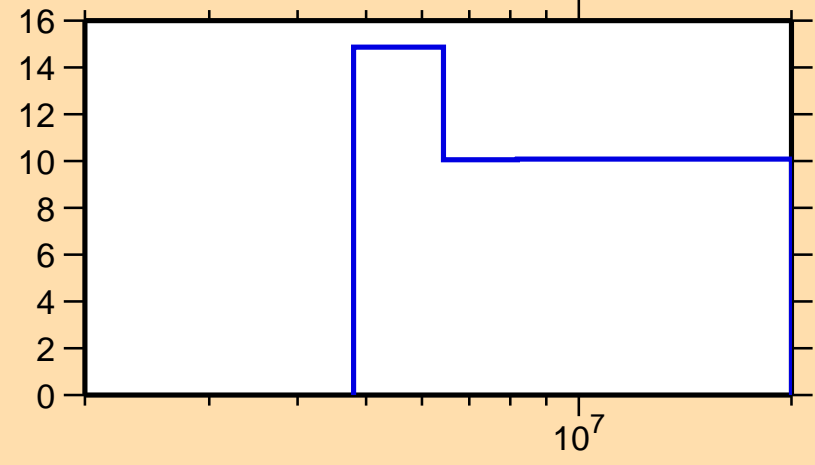
\Delta\sigma/\sigma vs. E for ^{213}\text{Bi}(n,\text{el.})
