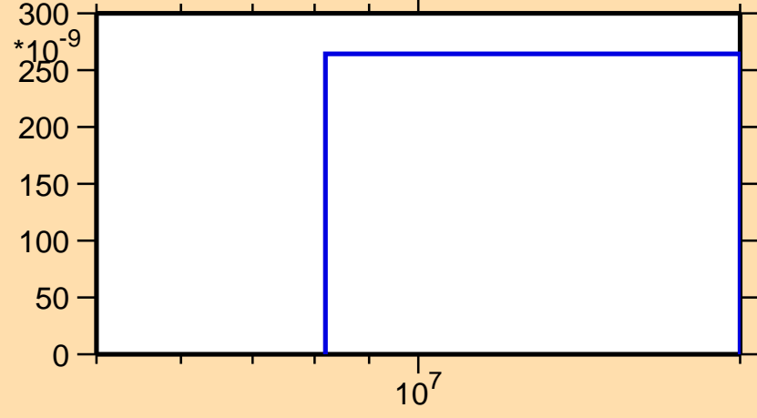
\sigma vs. E for ^{213}\text{Bi}(n,2np)
