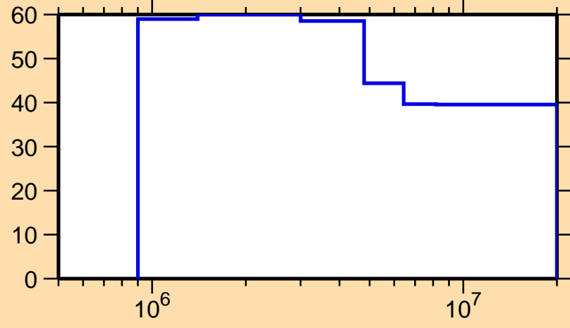
\Delta\sigma/\sigma vs. E for ^{213}\text{Bi}(n,n_1)
