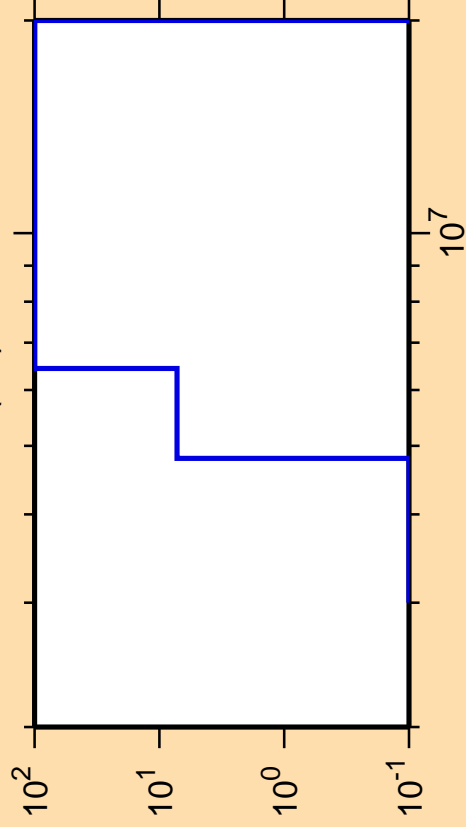
\Delta\sigma/\sigma vs. E for ^{213}\text{Bi}(n,t)
