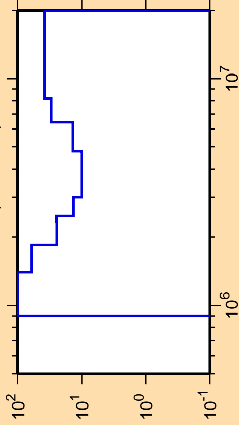
\Delta\sigma/\sigma vs. E for ^{213}\text{Bi}(n,n_{\text{cont}})
