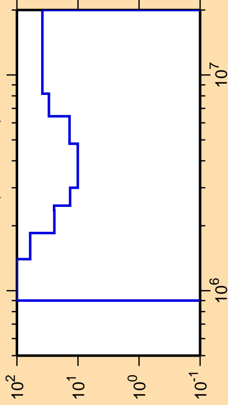
\Delta\sigma/\sigma vs. E for ^{213}\text{Bi}(n,\text{ncont.})
