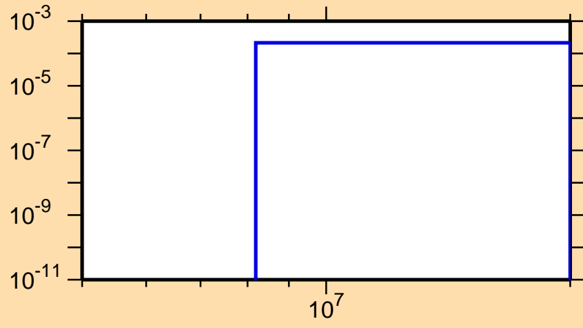
\sigma vs. E for ^{213}\text{Bi}(n,np)
