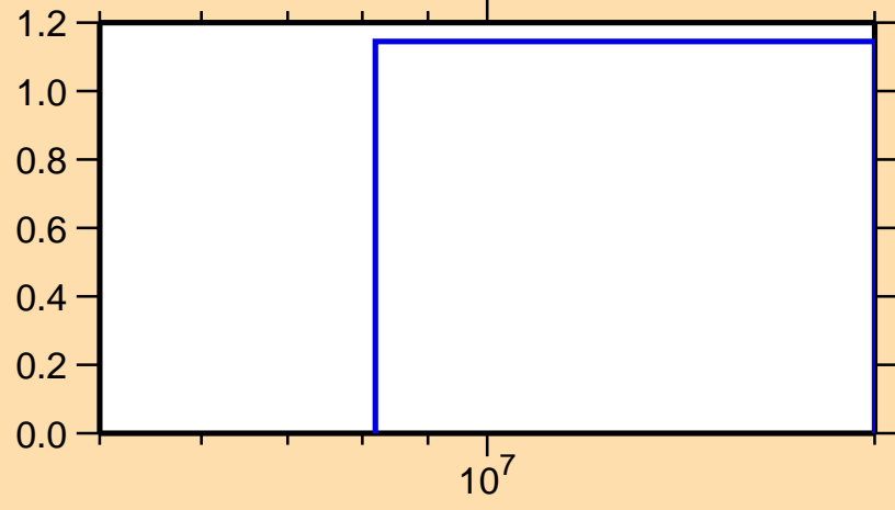
\sigma vs. E for ^{213}\text{Bi}(n,3n)
