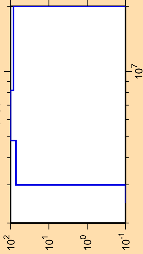
\Delta\sigma/\sigma vs. E for ^{213}\text{Bi}(n,p)
