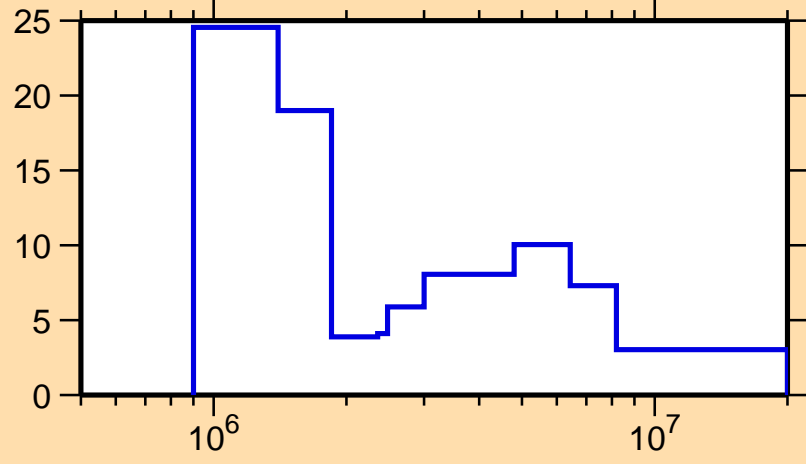
\Delta\sigma/\sigma vs. E for ^{213}\text{Bi}(n,\text{tot.})
