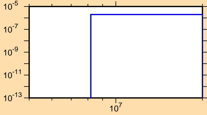
\sigma vs. E for ^{213}\text{Bi}(n,\text{nd})
