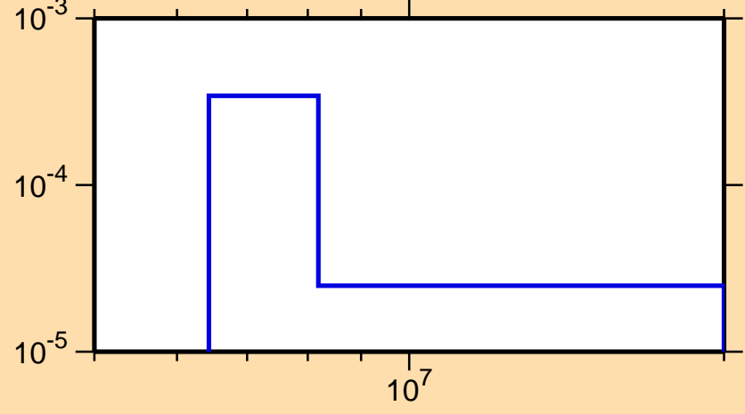
\sigma vs. E for ^{213}\text{Bi}(n,2n\alpha)
