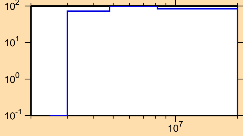
\Delta\sigma/\sigma vs. E for ^{213}\text{Bi}(n,p)
