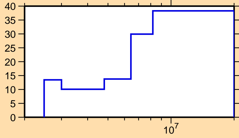
\Delta\sigma/\sigma vs. E for ^{213}\text{Bi}(n,n\text{cont.})
