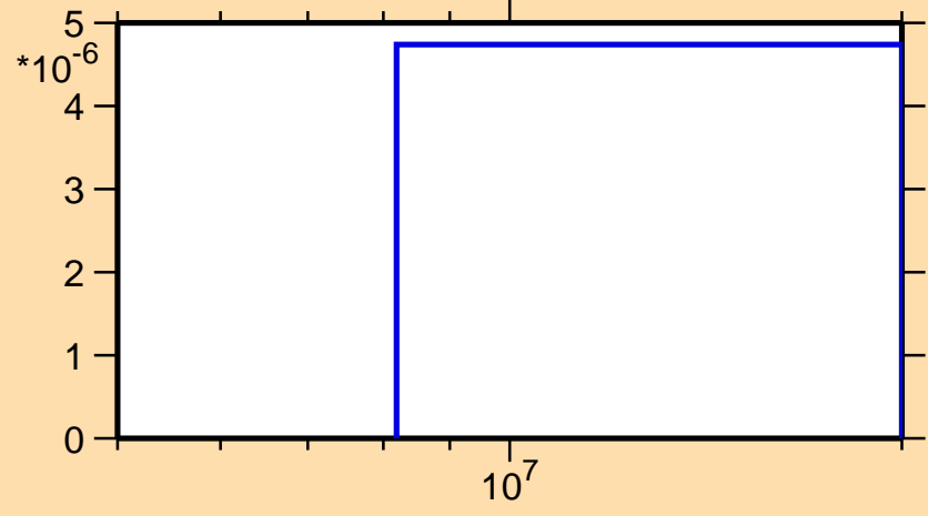
\sigma vs. E for ^{213}\text{Bi}(n,3n\alpha)
