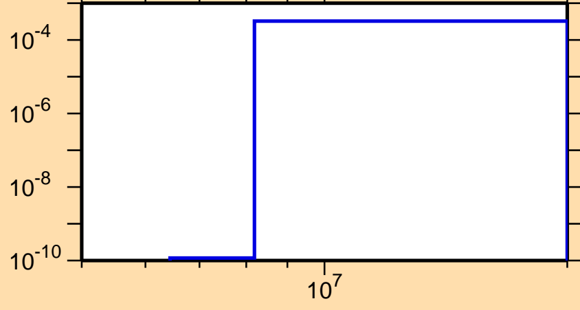
\sigma vs. E for ^{213}\text{Bi}(n,d)
