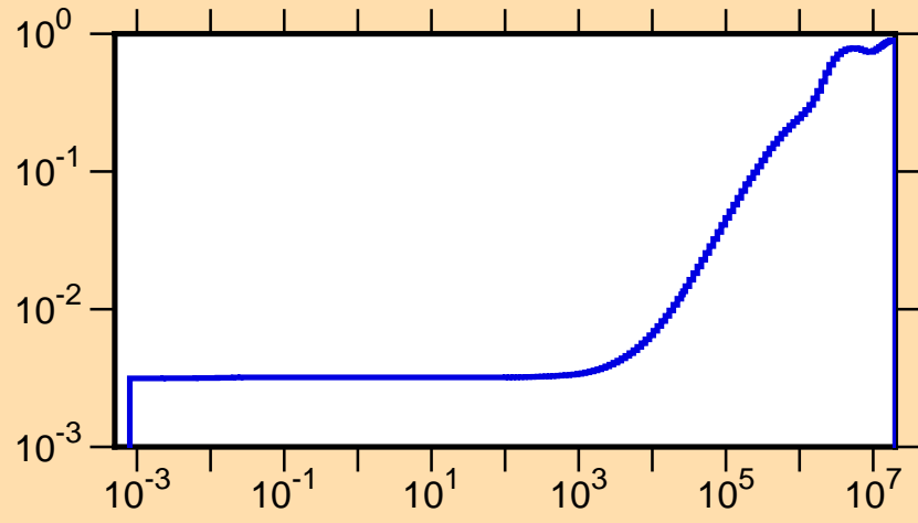
\mu vs. E for ^{214}\text{Bi}(\text{mt251})
