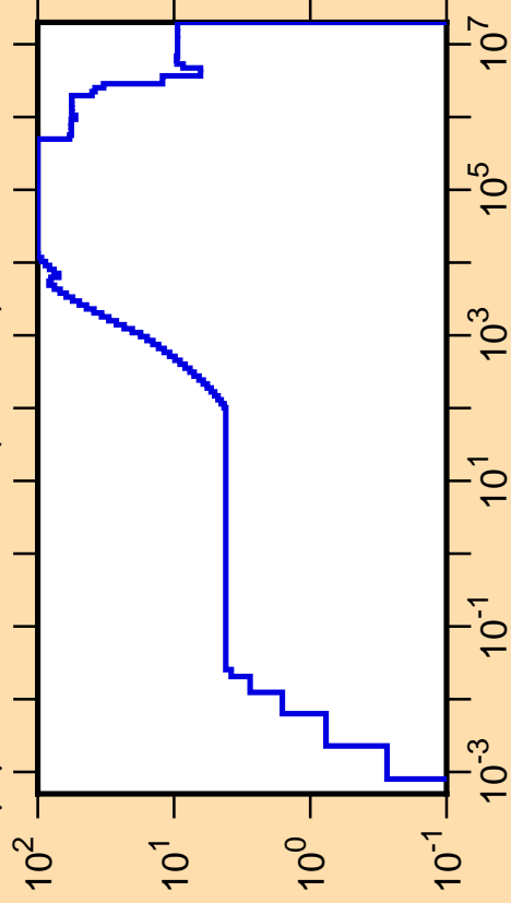
\Delta\mu/\mu vs. E for ^{214}\text{Bi}(\text{mt251})
