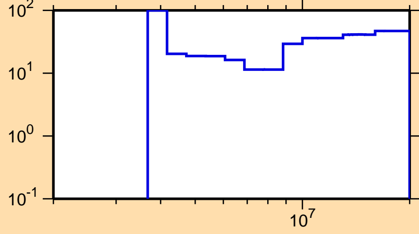
\Delta\sigma/\sigma vs. E for ^{214}\text{Bi}(n,2n)
