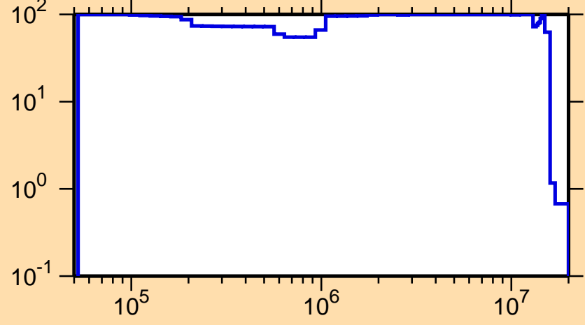
\Delta\sigma/\sigma vs. E for ^{214}\text{Bi}(n,n_1)
