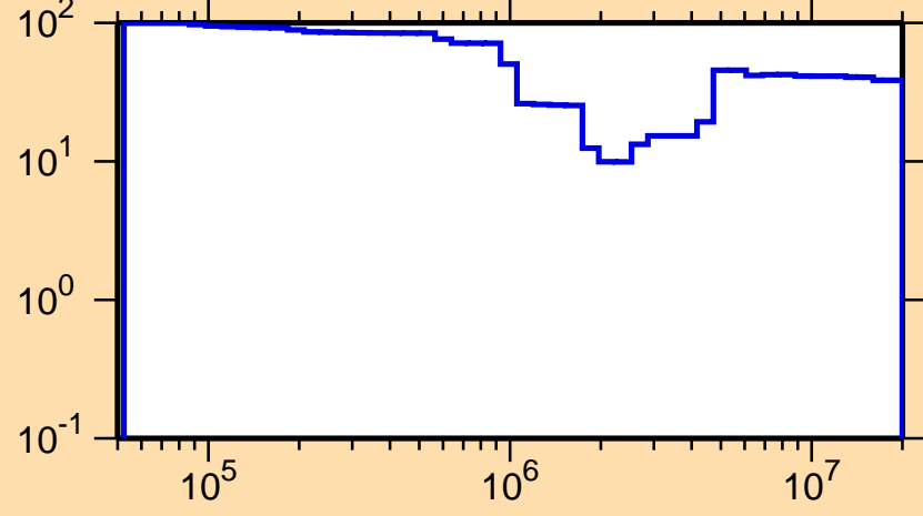
\Delta\sigma/\sigma vs. E for ^{214}\text{Bi}(n,\text{inel.})
