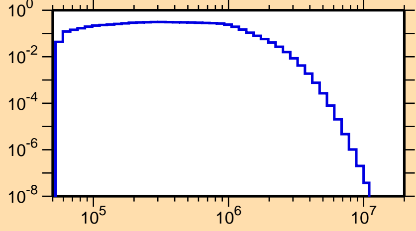
\sigma vs. E for ^{214}\text{Bi}(n,n_1)
