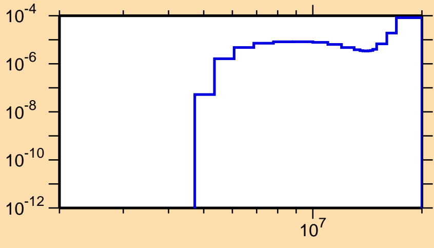
\sigma vs. E for ^{214}\text{Bi}(n,2n\alpha)
