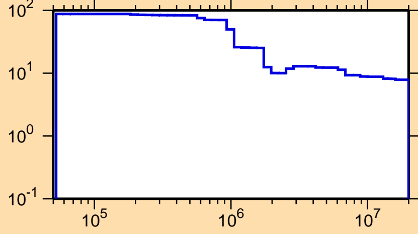
\Delta\sigma/\sigma vs. E for ^{214}\text{Bi}(n,\text{nonel.})
