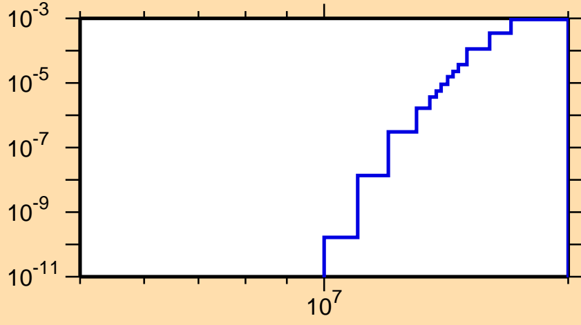
\sigma vs. E for ^{214}\text{Bi}(n,nt)
