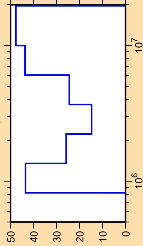
\Delta\sigma/\sigma vs. E for ^{214}\text{Bi}(n,\text{ncont.})
