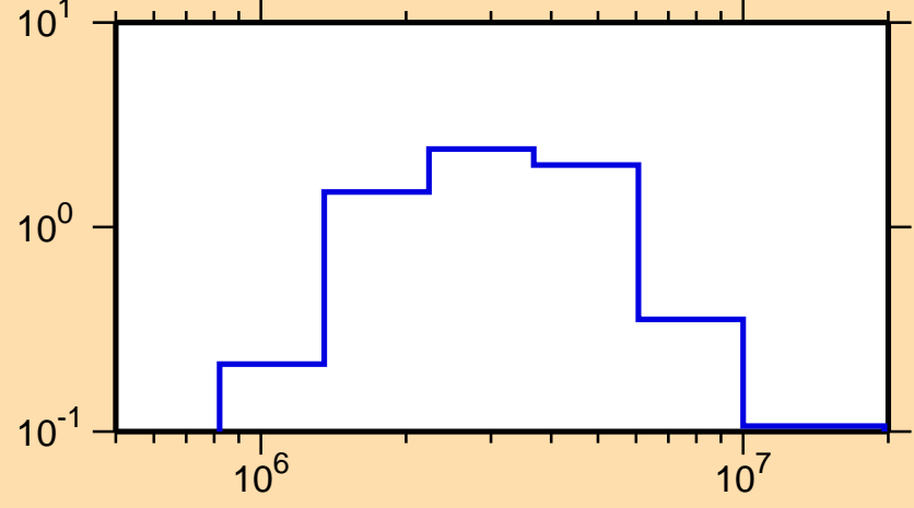
\sigma vs. E for ^{214}\text{Bi}(n,n\text{cont.})
