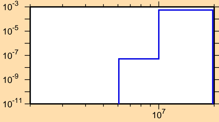
\sigma vs. E for ^{214}\text{Bi}(n,t)
