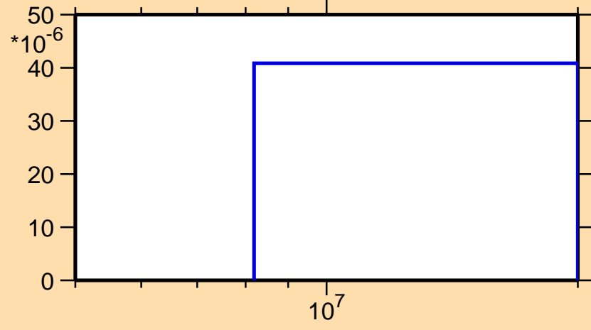
\sigma vs. E for ^{214}\text{Bi}(n,nt)
