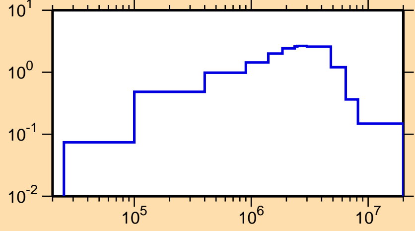
\sigma vs. E for ^{214}\text{Bi}(n,\text{inel.})
