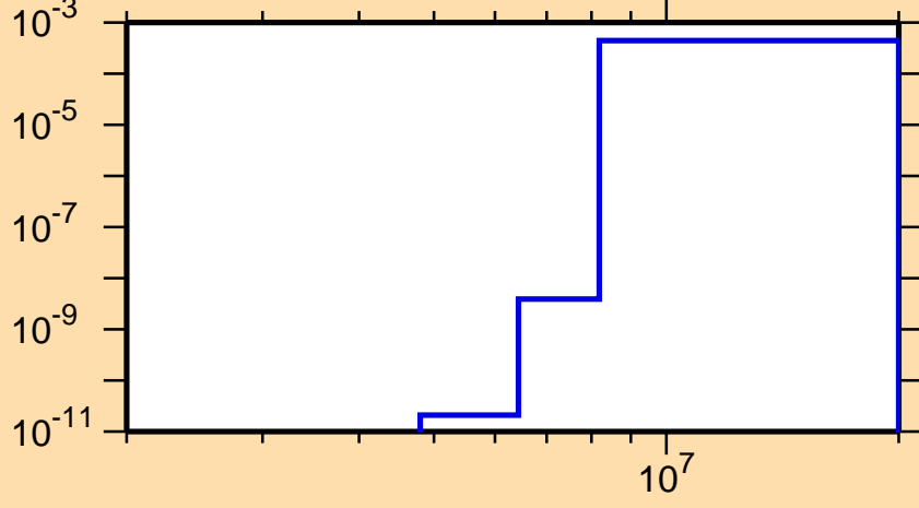
\sigma vs. E for ^{214}\text{Bi}(n,t)
