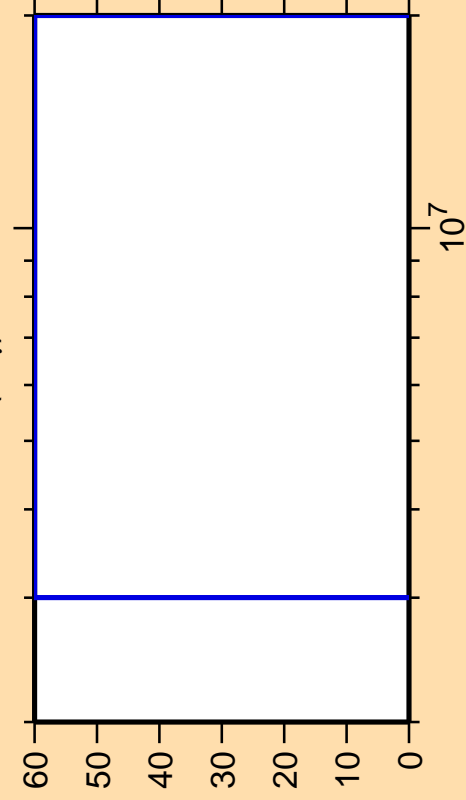
\Delta\sigma/\sigma vs. E for ^{214}\text{Bi}(n,\gamma)
