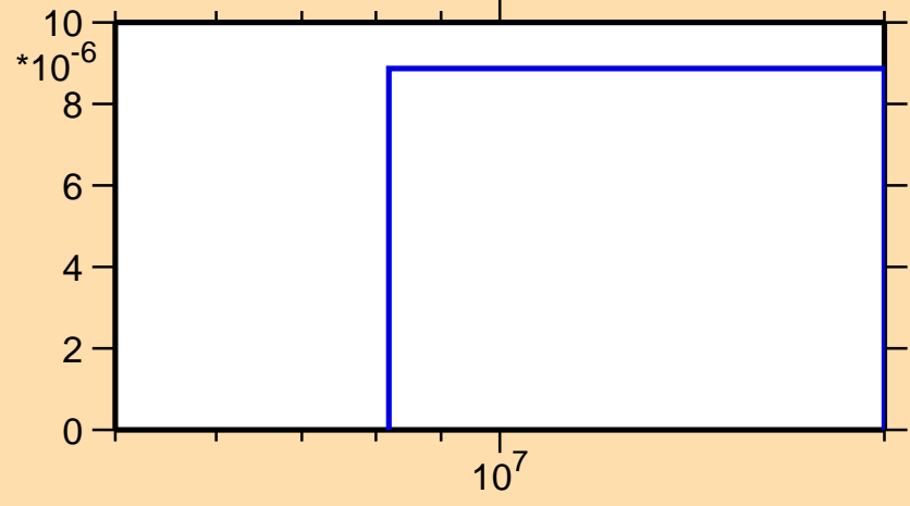
\sigma vs. E for ^{214}\text{Bi}(n,3n\alpha)
