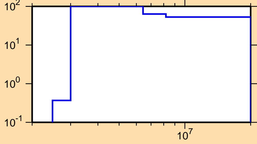
\Delta\sigma/\sigma vs. E for ^{214}\text{Bi}(n,p)
