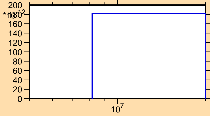
\sigma vs. E for ^{214}\text{Bi}(\text{mt } 11)
