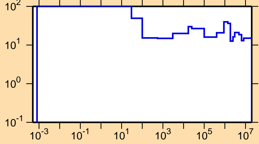
\Delta\sigma/\sigma vs. E for ^{214}\text{Bi}(n,\text{el.})
