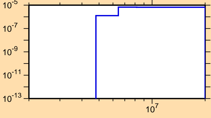
\sigma vs. E for ^{214}\text{Bi}(n,2n\alpha)
