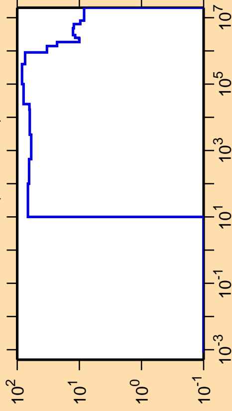
\Delta\sigma/\sigma vs. E for ^{214}\text{Bi}(n,\text{nonel.})
