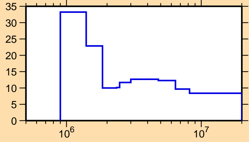
\Delta\sigma/\sigma vs. E for ^{214}\text{Bi}(n,n\text{onel.})
