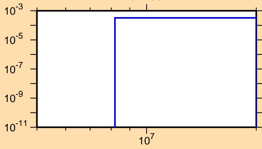
\sigma vs. E for ^{214}\text{Bi}(n,np)
