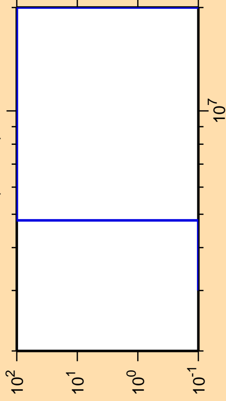
\Delta\sigma/\sigma vs. E for ^{214}\text{Bi}(n,2n\alpha)
