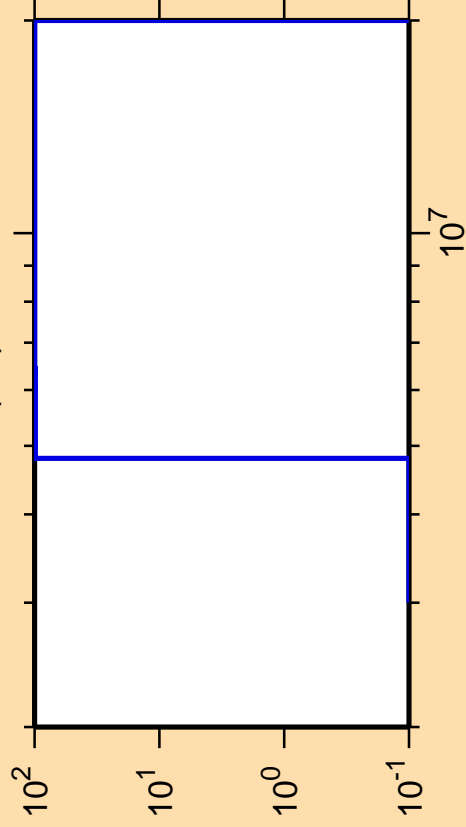
\Delta\sigma/\sigma vs. E for ^{214}\text{Bi}(n,t)
