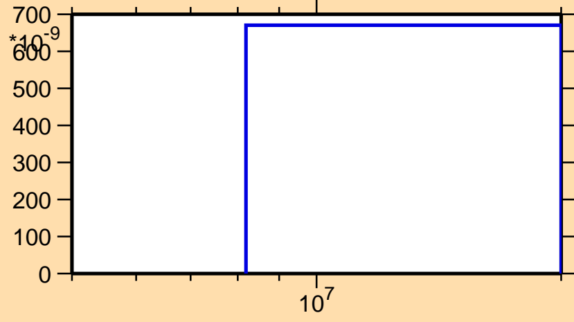
\sigma vs. E for ^{214}\text{Bi}(n,2np)
