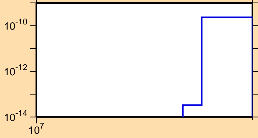
\sigma vs. E for ^{215}\text{Bi} (mt 42)
