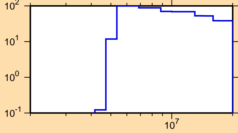
\Delta\sigma/\sigma vs. E for ^{215}\text{Bi}(n,p)
