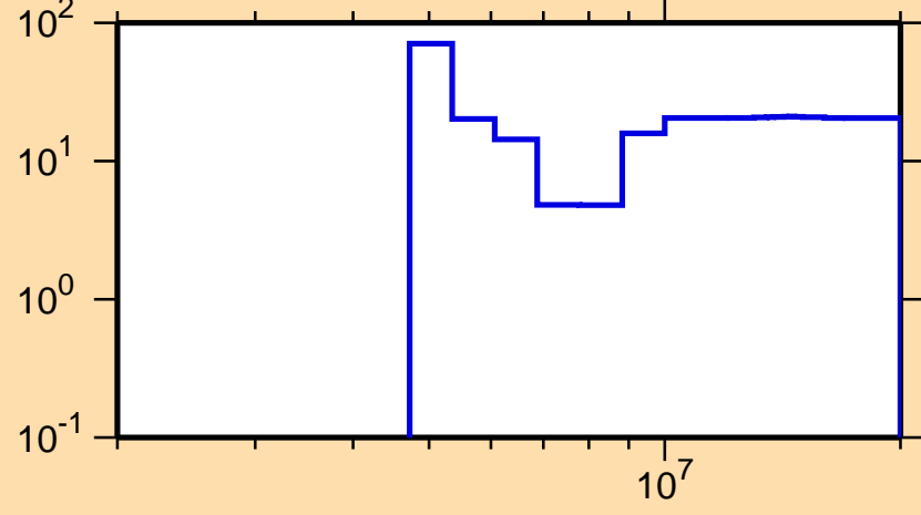
\Delta\sigma/\sigma vs. E for ^{215}\text{Bi}(n,2n)
