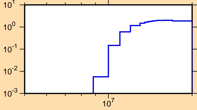
\sigma vs. E for ^{215}\text{Bi}(n,3n)
