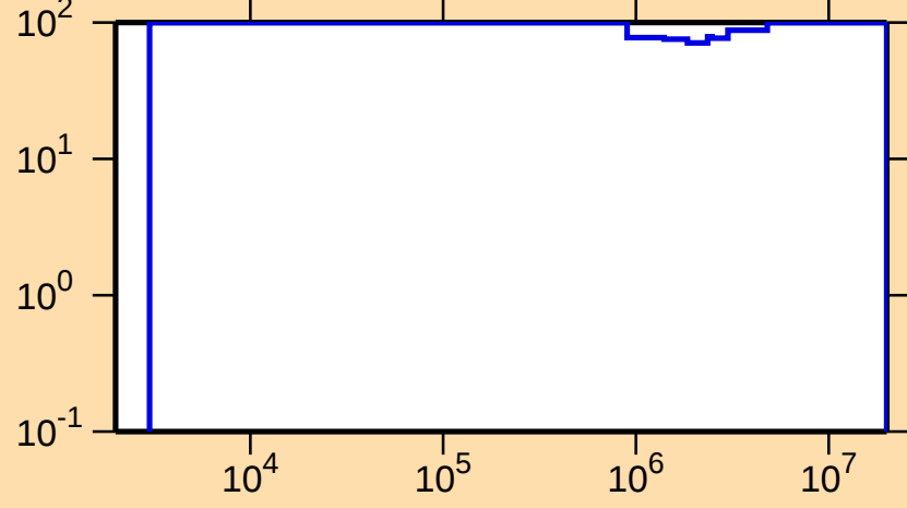
\Delta\sigma/\sigma vs. E for ^{215}\text{Bi}(n,n_1)
