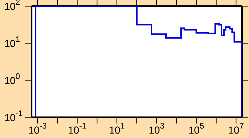
\Delta\sigma/\sigma vs. E for ^{215}\text{Bi}(n,\text{el.})
