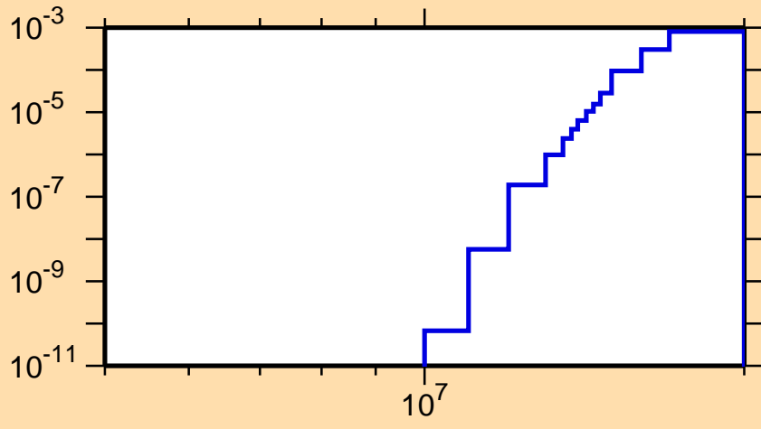
\sigma vs. E for ^{216}\text{Bi}(n,\text{nt})
