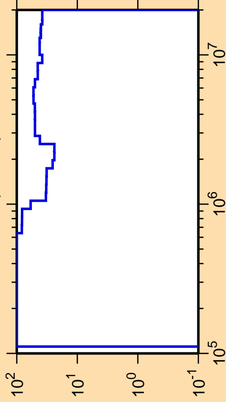
\Delta\sigma/\sigma vs. E for ^{216}\text{Bi}(n,\text{inel.})
