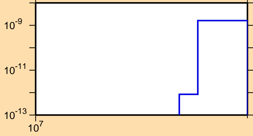
\sigma vs. E for ^{216}\text{Bi} (mt 42)
