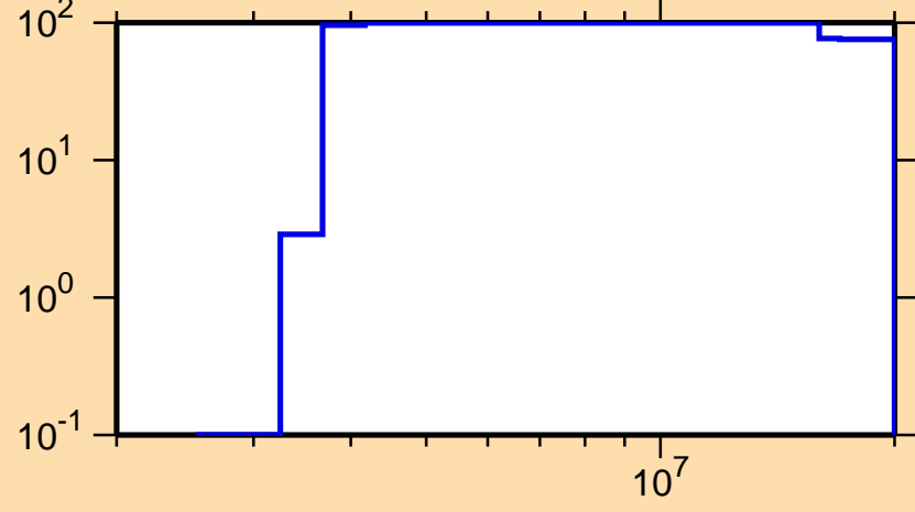
\Delta\sigma/\sigma vs. E for ^{216}\text{Bi}(n,p)
