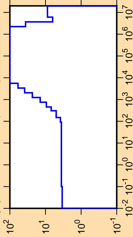
\Delta\mu/\mu vs. E for ^{216}\text{Bi}(\text{mt251})
