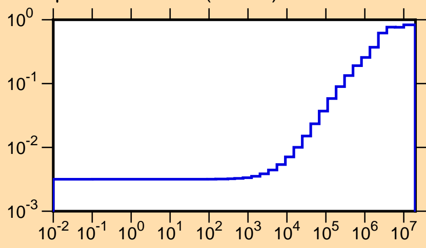
\mu vs. E for ^{216}\text{Bi}(\text{mt251})
