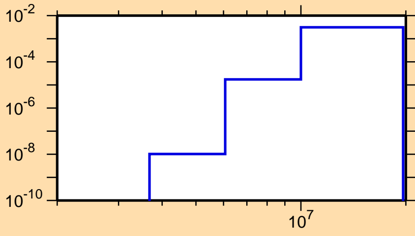
\sigma vs. E for ^{216}\text{Bi}(n,p)
