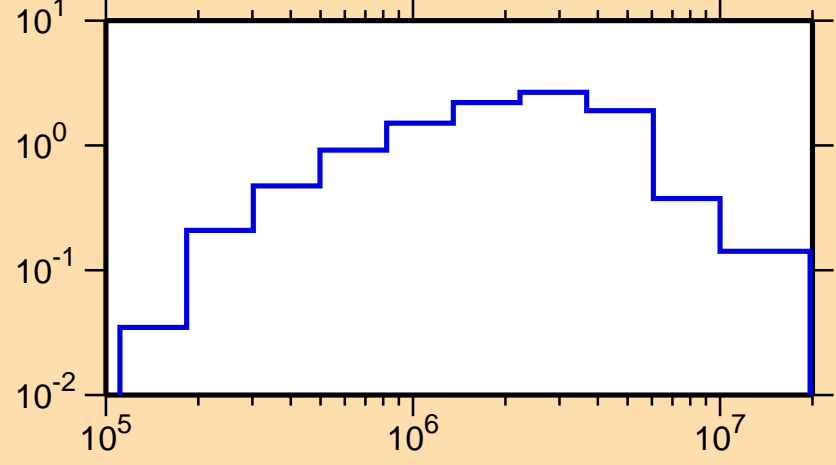
\sigma vs. E for ^{216}\text{Bi}(n,\text{inel.})
