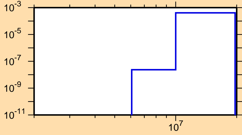
\sigma vs. E for ^{216}\text{Bi}(n,t)
