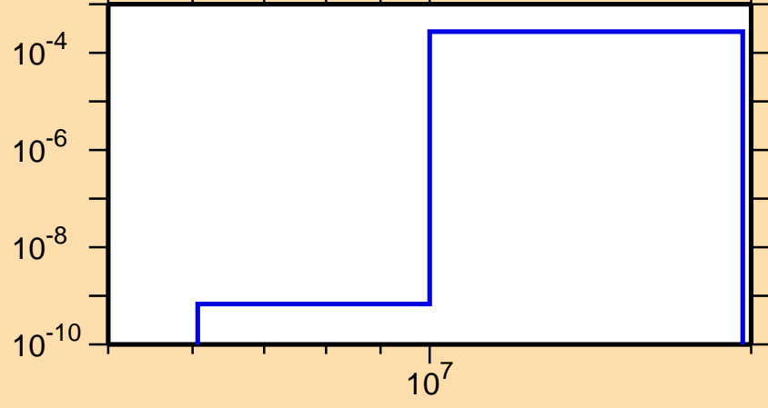
\sigma vs. E for ^{216}\text{Bi}(n,d)
