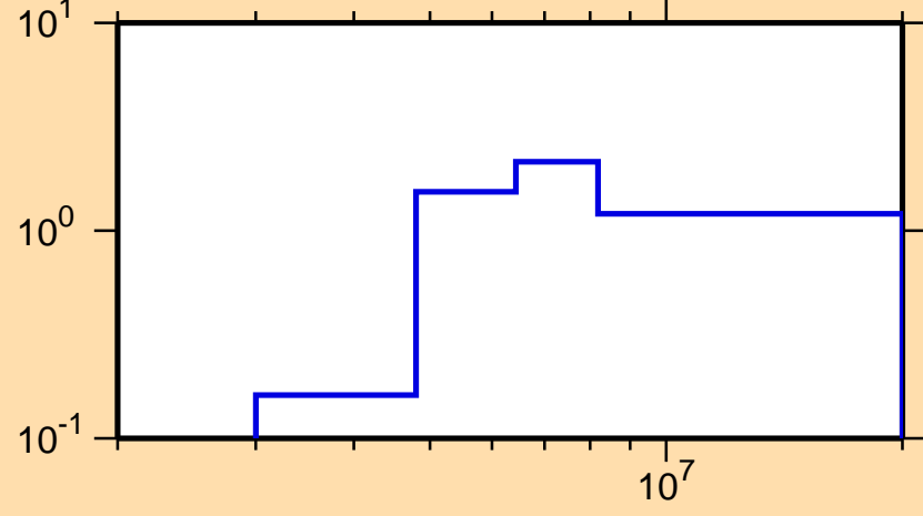
\sigma vs. E for ^{216}\text{Bi}(n,2n)
