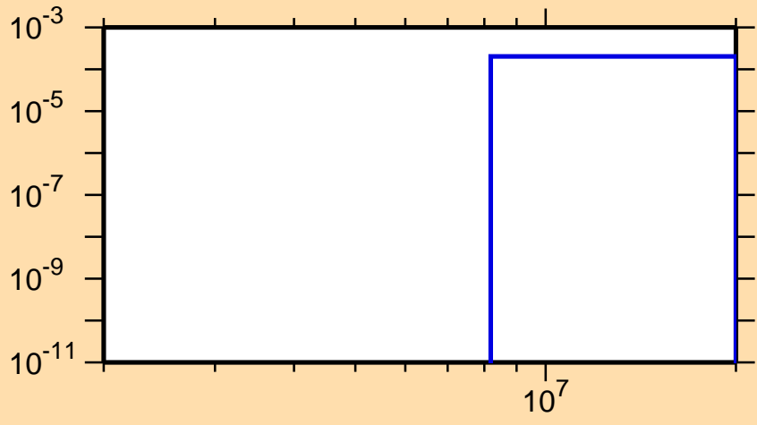
\sigma vs. E for ^{216}\text{Bi}(n,np)
