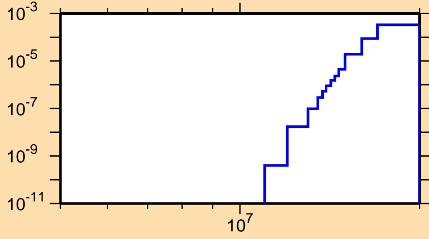
\sigma vs. E for ^{217}\text{Bi}(n,nt)
