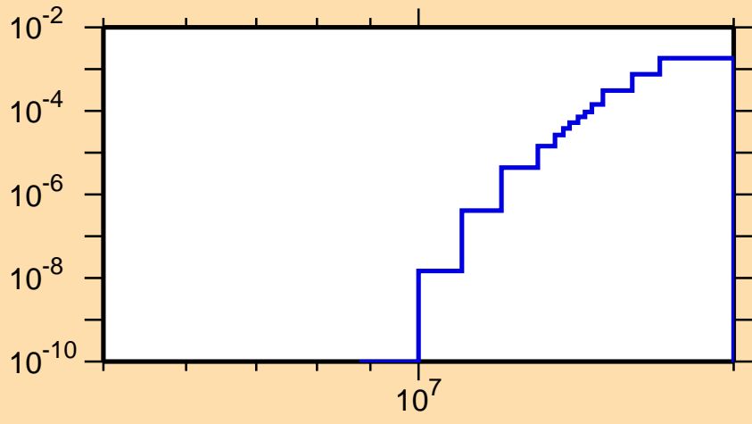
\sigma vs. E for ^{217}\text{Bi}(n,np)
