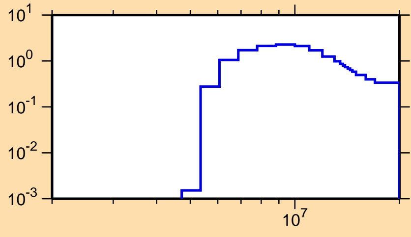
\sigma vs. E for ^{217}\text{Bi}(n,2n)
