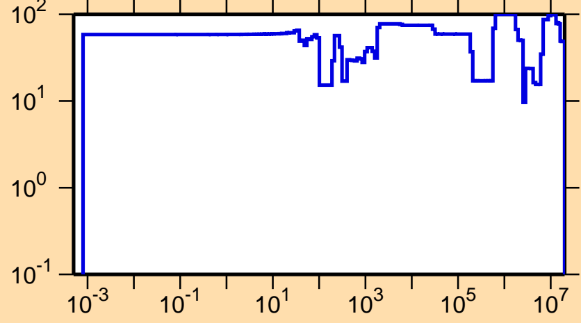
\Delta\sigma/\sigma vs. E for ^{217}\text{Bi}(n,\text{el.})
