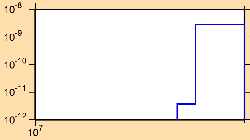
\sigma vs. E for ^{217}\text{Bi} (mt 11)
