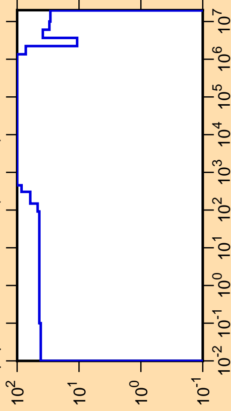
\Delta\mu/\mu vs. E for ^{217}\text{Bi}(\text{mt251})
