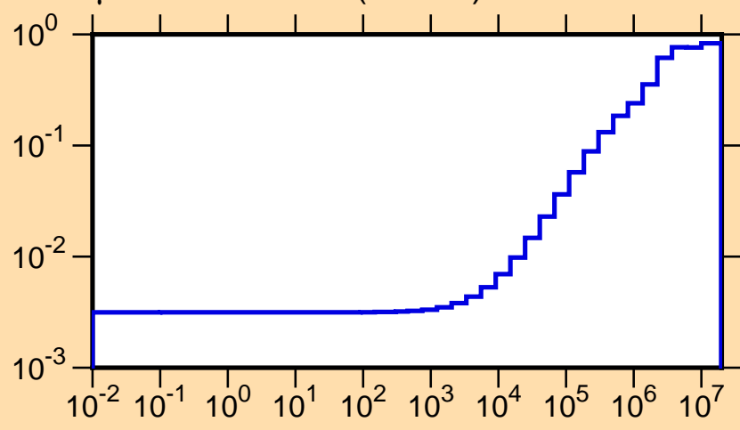
\mu vs. E for ^{217}\text{Bi}(\text{mt251})
