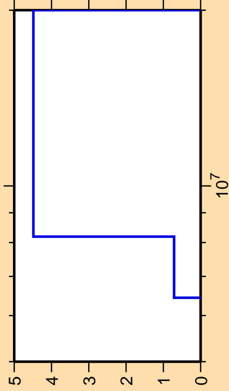
\Delta\sigma/\sigma vs. E for ^{217}\text{Bi}(n,t)
