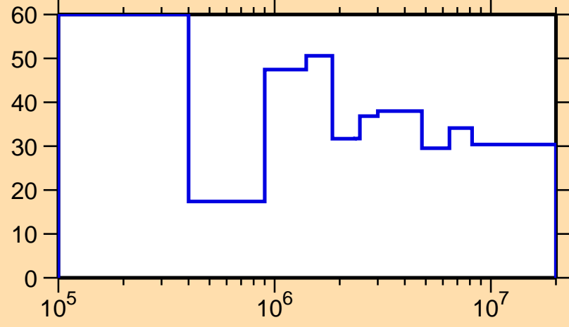
\Delta\sigma/\sigma vs. E for ^{217}\text{Bi}(n,n\text{onel.})
