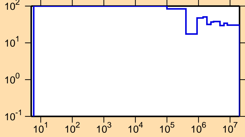
\Delta\sigma/\sigma vs. E for ^{217}\text{Bi}(n,\text{nonel.})
