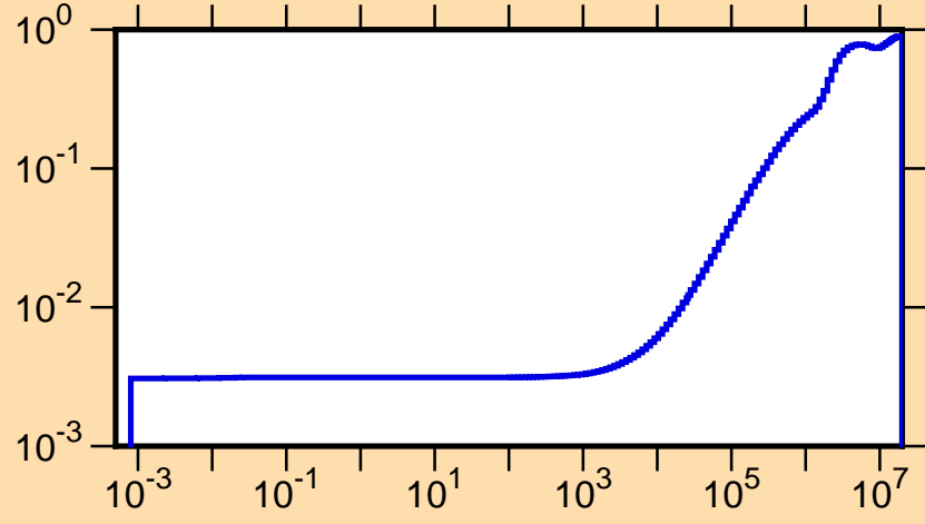
\mu vs. E for ^{219}\text{Bi}(\text{mt251})
