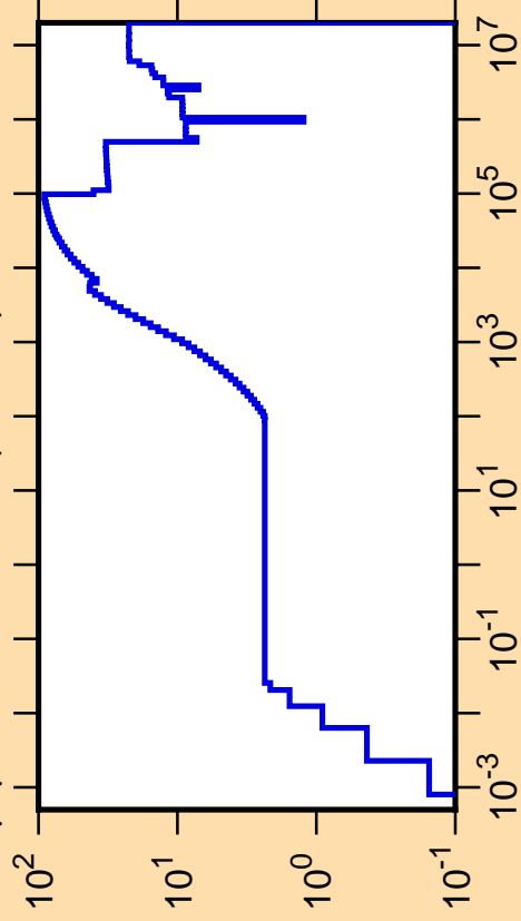
\Delta\mu/\mu vs. E for ^{219}\text{Bi}(\text{mt251})
