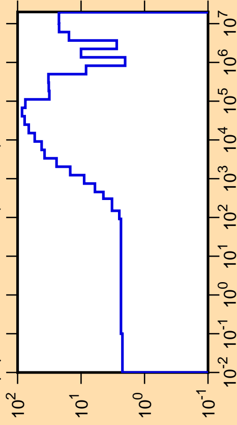
\Delta\mu/\mu vs. E for ^{219}\text{Bi}(\text{mt251})
