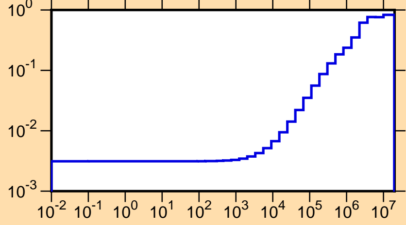
\mu vs. E for ^{219}\text{Bi}(\text{mt251})
