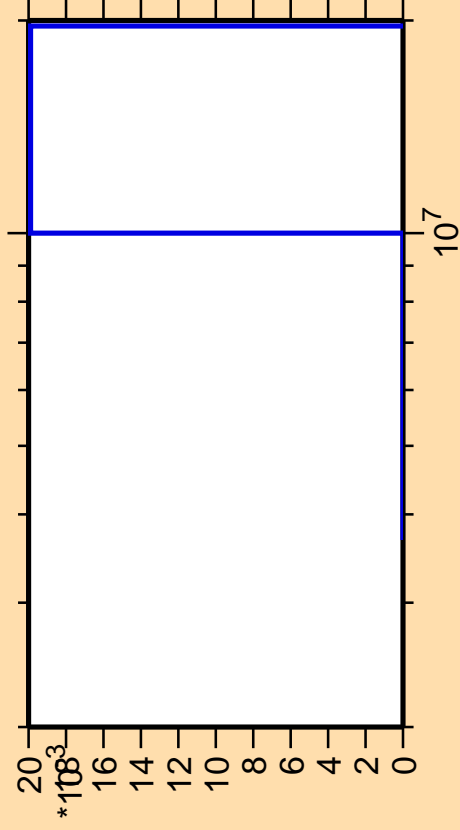
\Delta\sigma/\sigma vs. E for ^{219}\text{Bi}(n,f)
