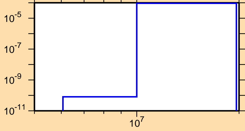
\sigma vs. E for ^{219}\text{Bi}(n,d)
