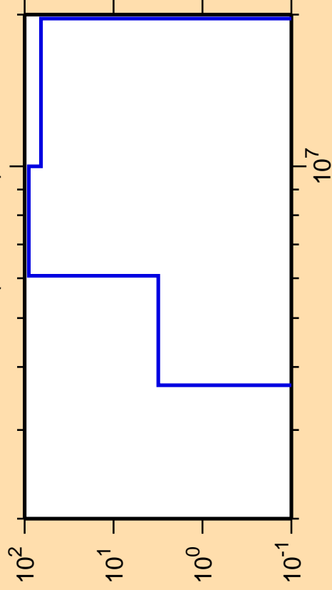
\Delta\sigma/\sigma vs. E for ^{219}\text{Bi}(n,\text{ncont.})
