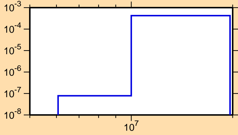
\sigma vs. E for ^{219}\text{Bi}(n,p)
