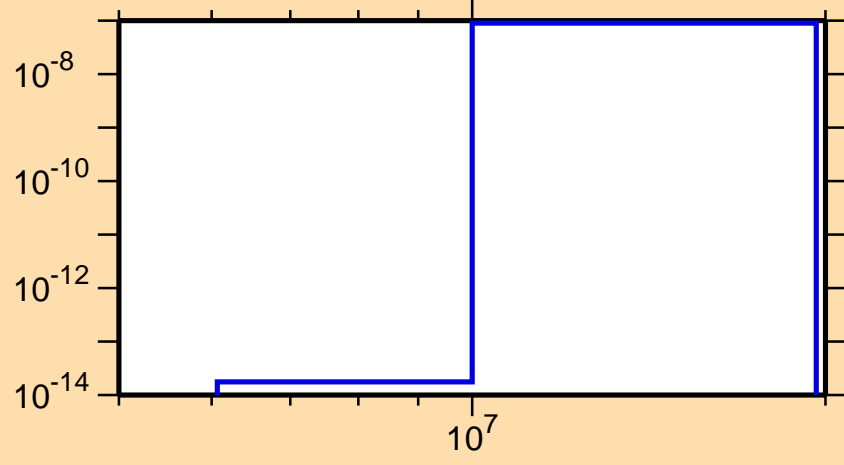
\sigma vs. E for ^{219}\text{Bi}(n,2n\alpha)
