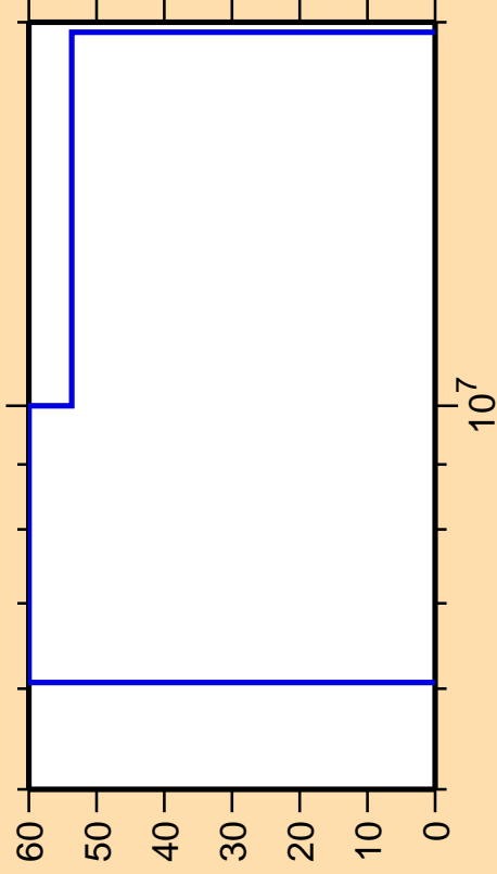
\Delta\sigma/\sigma vs. E for ^{219}\text{Bi}(n,d)
