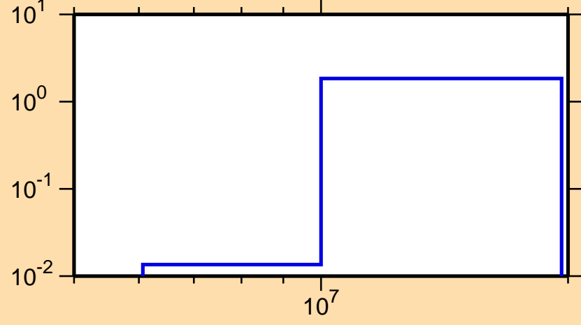
\sigma vs. E for ^{219}\text{Bi}(n,3n)
