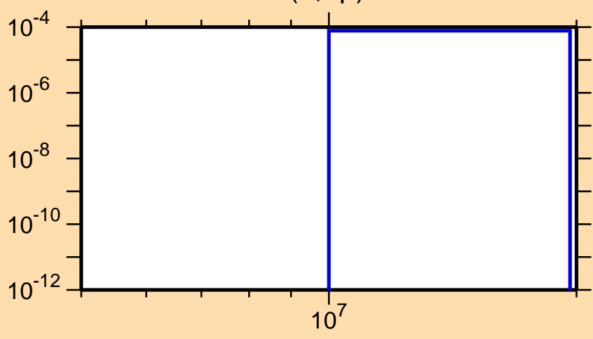
\sigma vs. E for ^{219}\text{Bi}(n,np)
