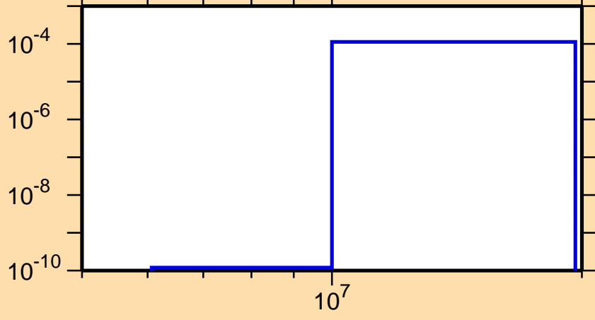
\sigma vs. E for ^{219}\text{Bi}(n,t)
