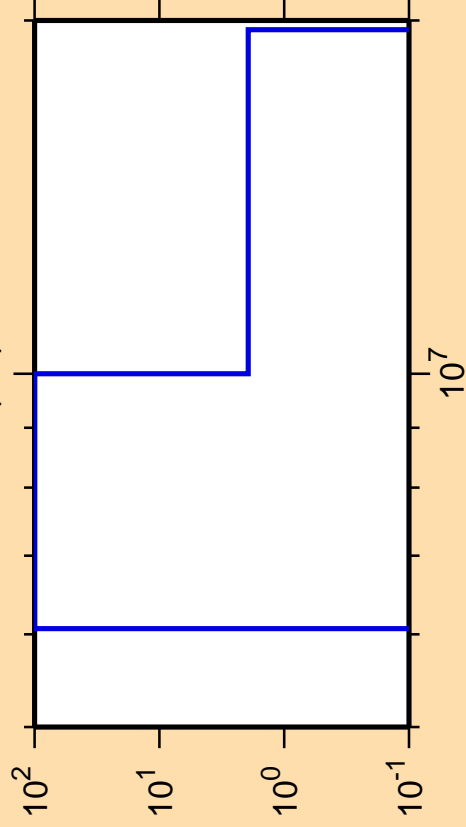
\Delta\sigma/\sigma vs. E for ^{219}\text{Bi}(n,t)
