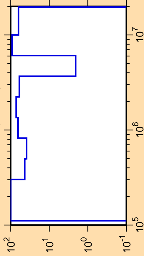
\Delta\sigma/\sigma vs. E for ^{219}\text{Bi}(n,\text{inel.})
