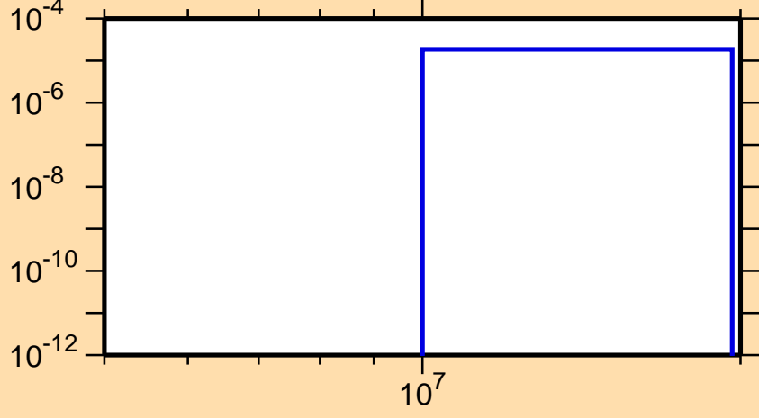
\sigma vs. E for ^{219}\text{Bi}(n,nt)
