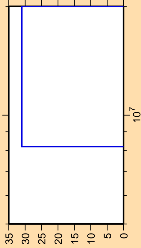
\Delta\sigma/\sigma vs. E for ^{219}\text{Bi}(\text{mt } 11)
