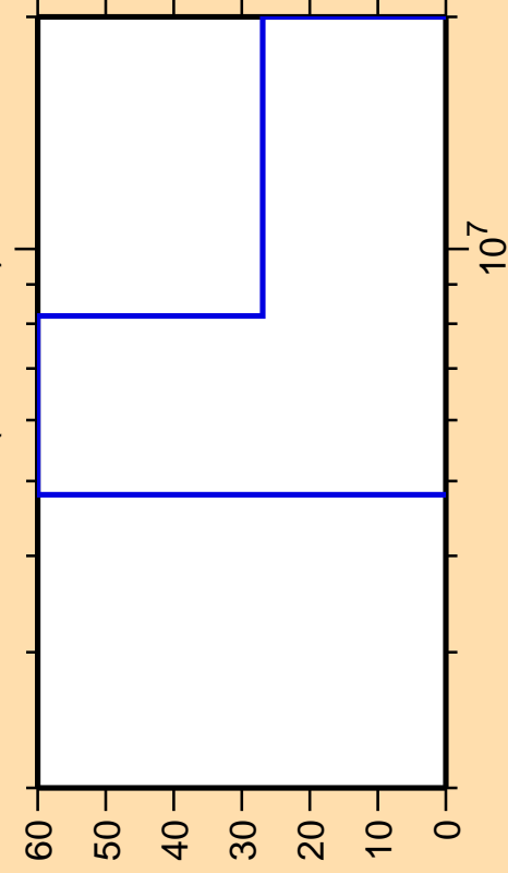
\Delta\sigma/\sigma vs. E for ^{219}\text{Bi}(n,n\text{cont.})
