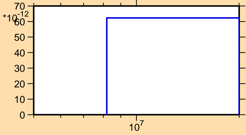
\sigma vs. E for ^{219}\text{Bi}(\text{mt } 11)
