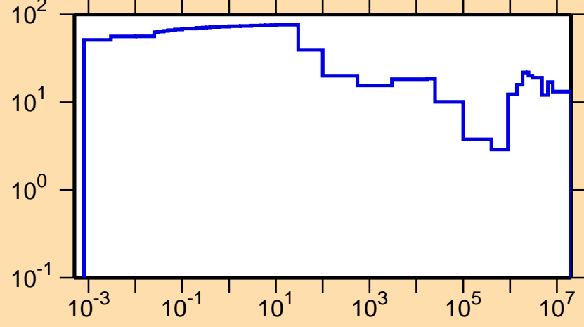
\Delta\sigma/\sigma vs. E for ^{219}\text{Bi}(n,\text{tot.})
