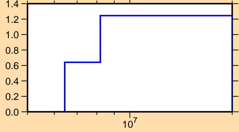
\Delta\sigma/\sigma vs. E for ^{219}\text{Bi}(n,el.)
