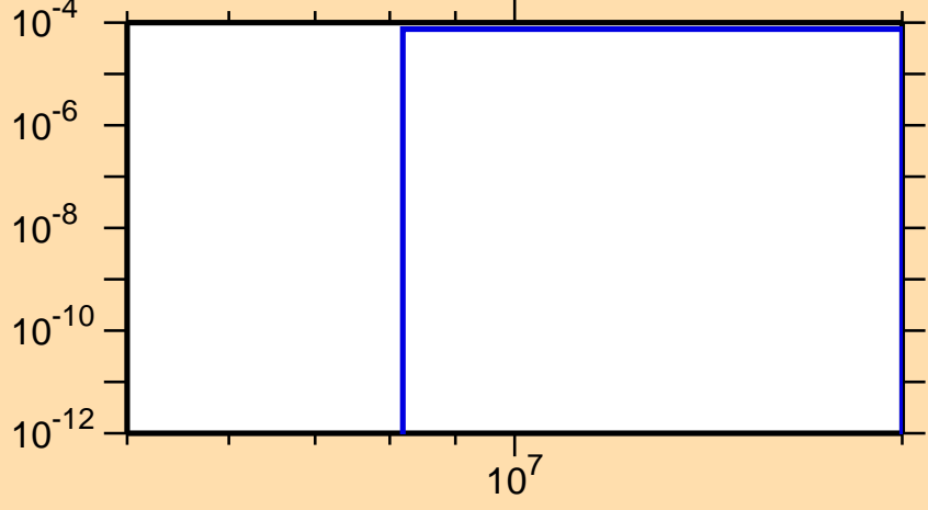
\sigma vs. E for ^{219}\text{Bi}(n,d)
