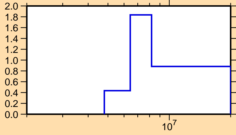
\sigma vs. E for ^{219}\text{Bi}(n,2n)
