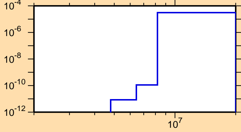
\sigma vs. E for ^{219}\text{Bi}(n,\alpha)
