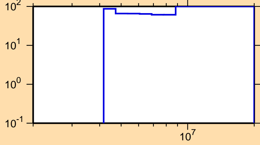
\Delta\sigma/\sigma vs. E for ^{220}\text{Bi}(n,2n)
