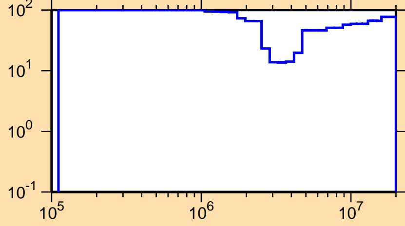
\Delta\sigma/\sigma vs. E for ^{220}\text{Bi}(n,\text{inel.})
