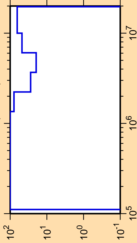
\Delta\sigma/\sigma vs. E for ^{220}\text{Bi}(n,\text{inel.})
