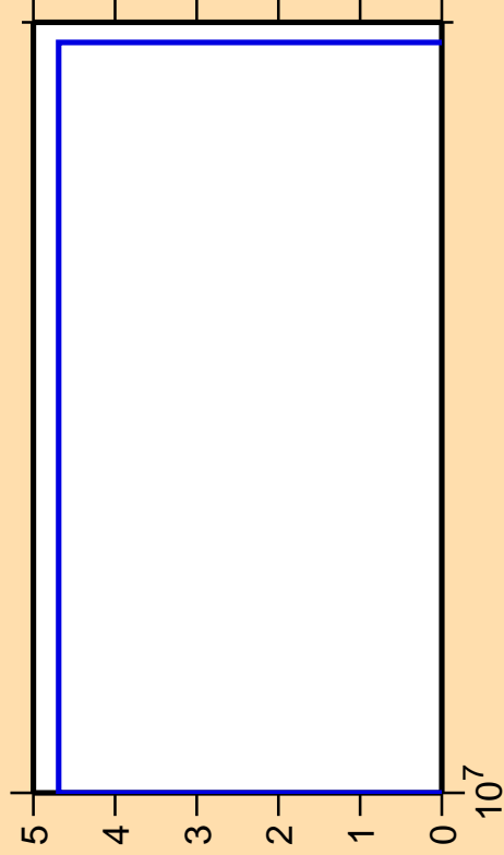
\Delta\sigma/\sigma vs. E for ^{220}\text{Bi} (mt 42)
