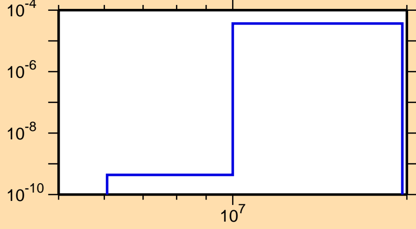
\sigma vs. E for ^{220}\text{Bi}(n,\alpha)
