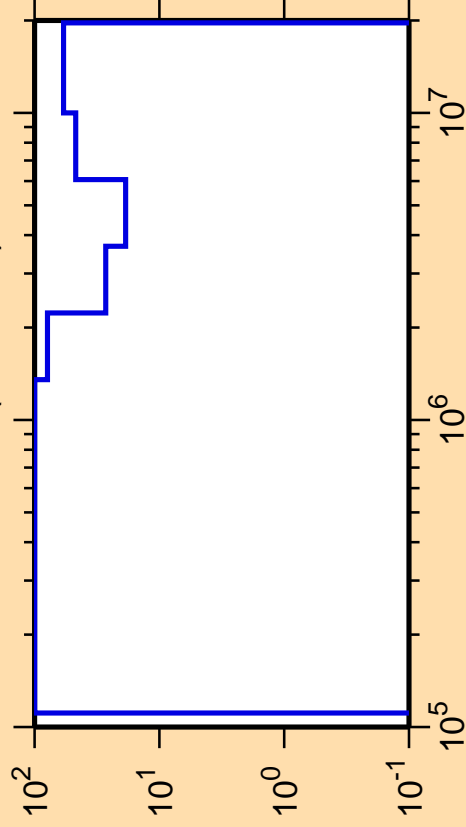
\Delta\sigma/\sigma vs. E for ^{220}\text{Bi}(n,\text{ncont.})
