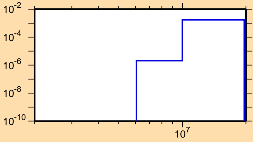
\sigma vs. E for ^{220}\text{Bi}(n,p)
