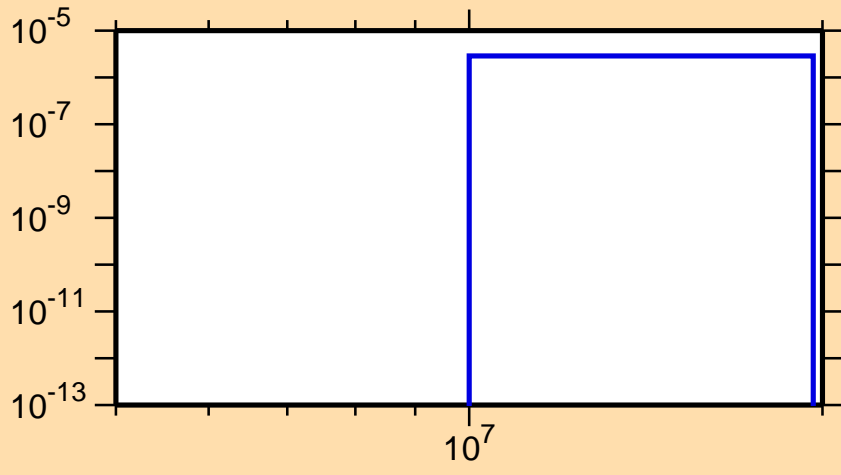
\sigma vs. E for ^{220}\text{Bi}(n,\text{nd})
