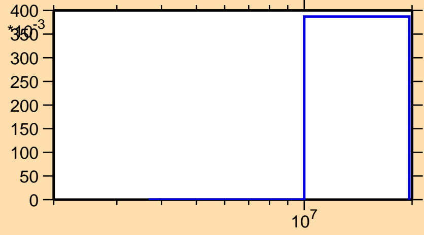
\Delta\sigma/\sigma vs. E for ^{220}\text{Bi}(n,f)
