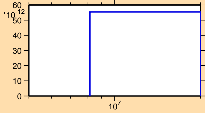
\sigma vs. E for ^{220}\text{Bi}(\text{mt } 11)
