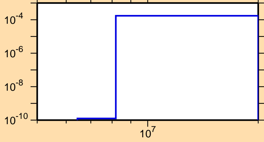
\sigma vs. E for ^{220}\text{Bi}(n,t)
