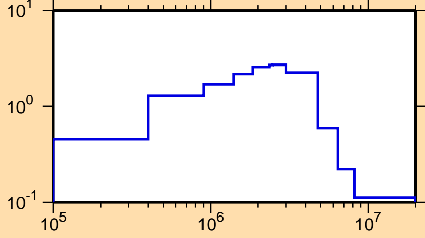
\sigma vs. E for ^{220}\text{Bi}(n,\text{inel.})
