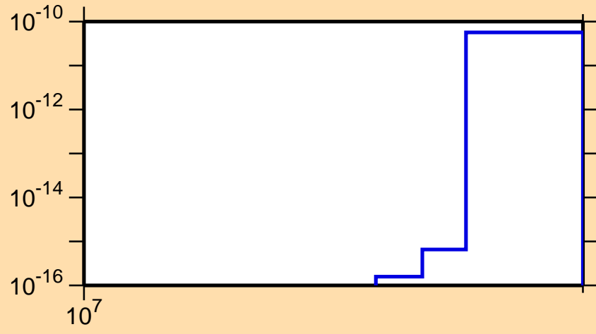
\sigma vs. E for ^{221}\text{Bi} (mt 42)
