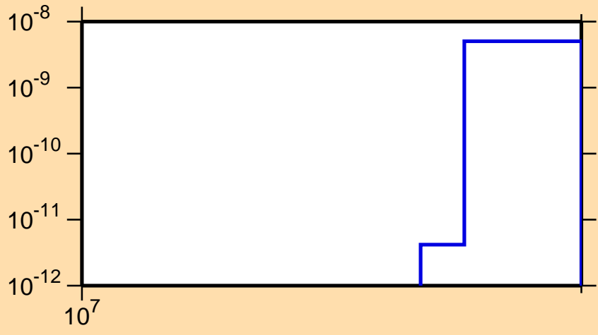
\sigma vs. E for ^{221}\text{Bi} (mt 11)
