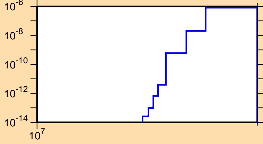
\sigma vs. E for ^{221}\text{Bi}(n,2np)
