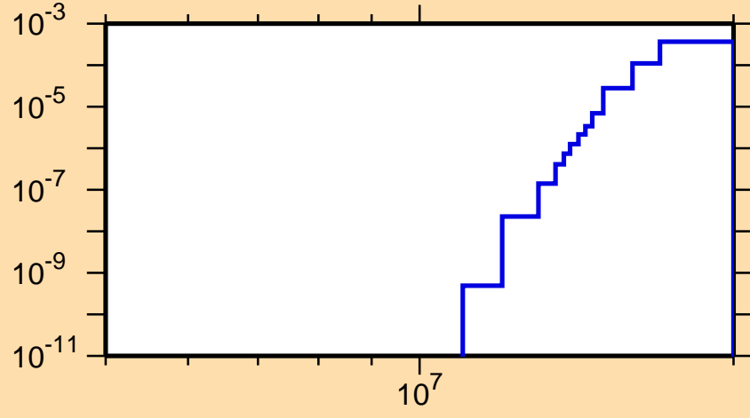
\sigma vs. E for ^{221}\text{Bi}(n,\text{nt})
