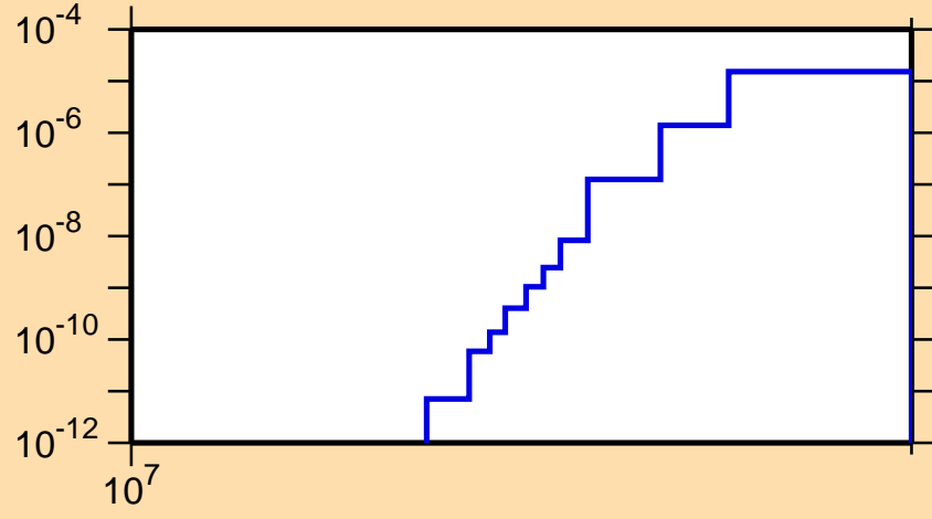
\sigma vs. E for ^{221}\text{Bi}(n,\text{nd})
