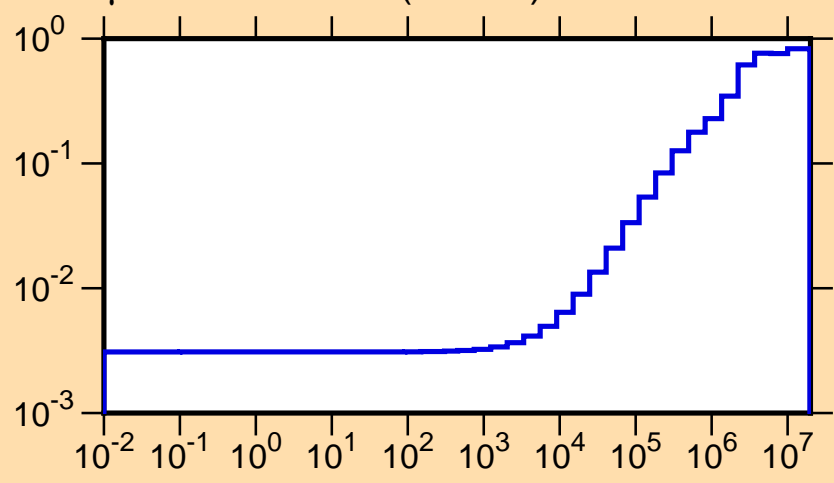
\mu vs. E for ^{221}\text{Bi}(\text{mt251})
