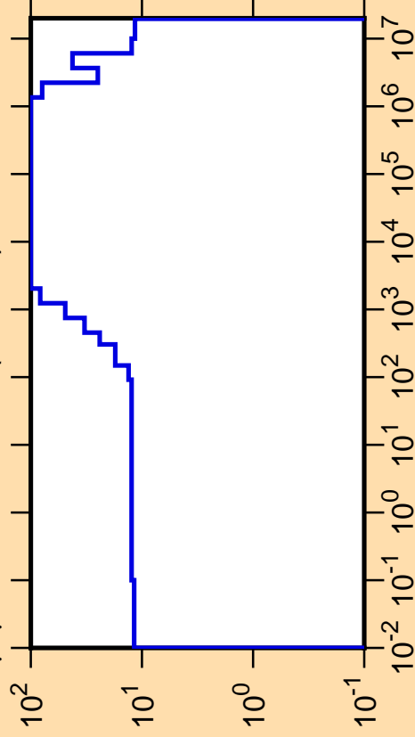
\Delta\mu/\mu vs. E for ^{221}\text{Bi}(\text{mt251})
