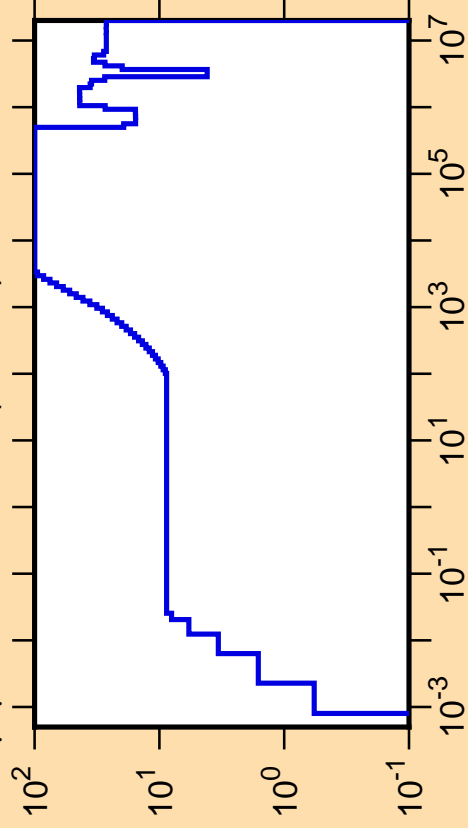
\Delta\mu/\mu vs. E for ^{222}\text{Bi}(\text{mt251})
