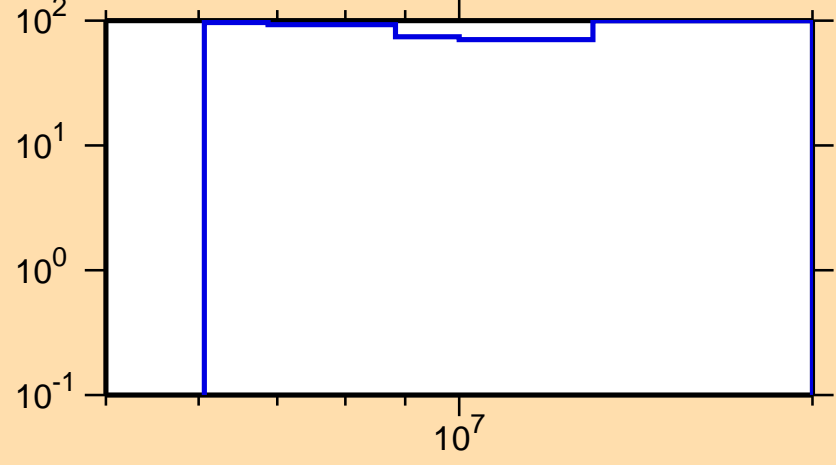
\Delta\sigma/\sigma vs. E for ^{222}\text{Bi}(n,\gamma)
