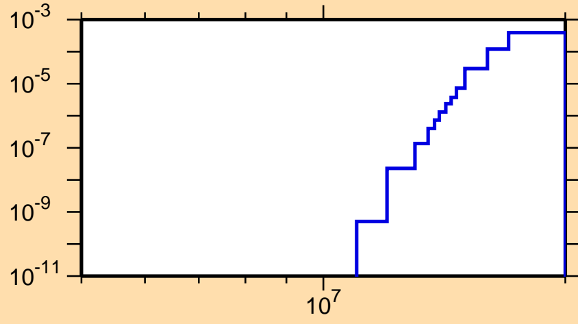
\sigma vs. E for ^{222}\text{Bi}(n,\text{nt})
