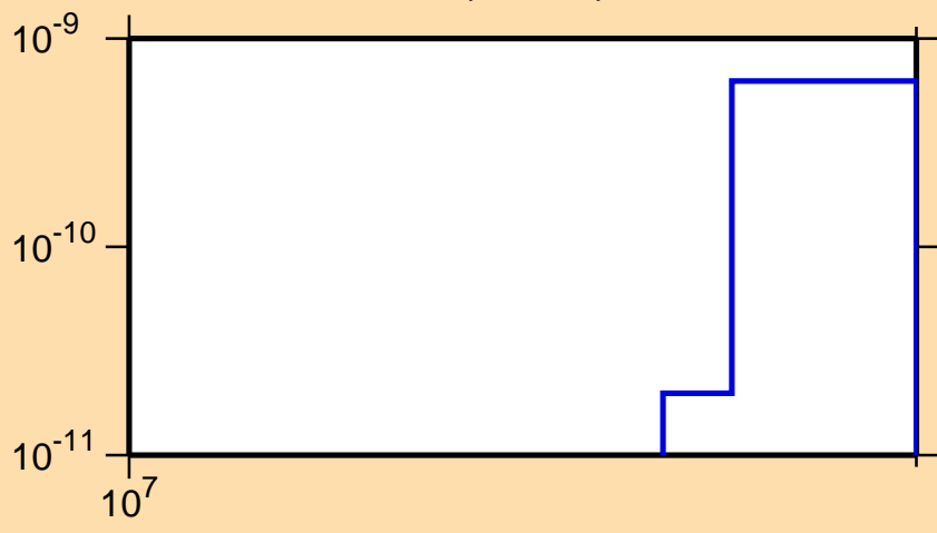
\sigma vs. E for ^{222}\text{Bi}(n,3n\alpha)
