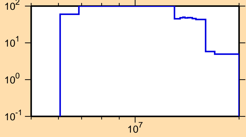
\Delta\sigma/\sigma vs. E for ^{222}\text{Bi}(n,el.)
