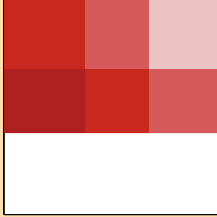
\Delta\sigma/\sigma vs. E for ^{70}\text{Br}(n,\text{el.})
