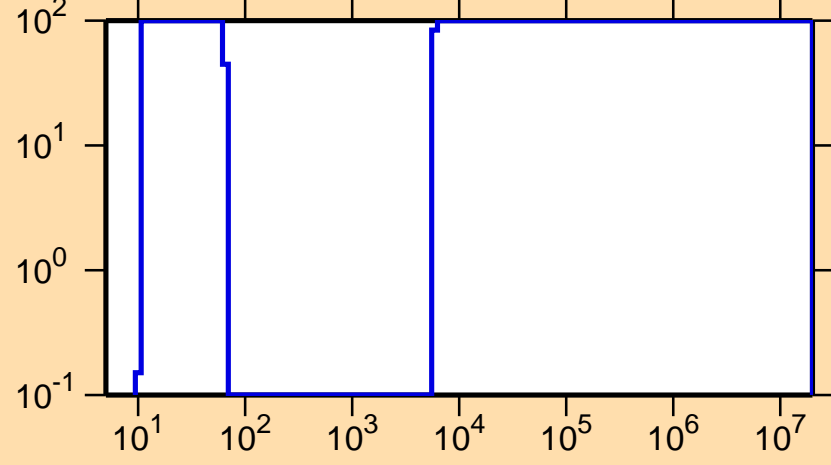
\Delta\sigma/\sigma vs. E for ^{70}\text{Br}(n,n\text{cont.})
