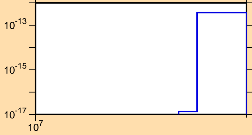
\sigma vs. E for ^{70}\text{Br}(n,2n\alpha)
