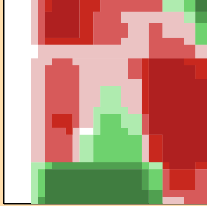
\Delta\sigma/\sigma vs. E for ^{76}\text{Br}(n,n\text{cont.})
