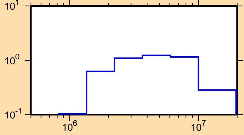
\sigma vs. E for ^{76}\text{Br}(n,n\text{cont.})
