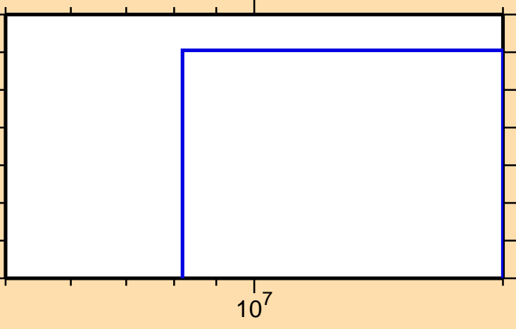
\sigma vs. E for ^{77}\text{Br}(n,2np)
