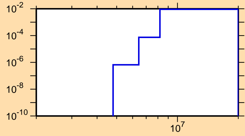
\sigma vs. E for ^{77}\text{Br}(n,d)
