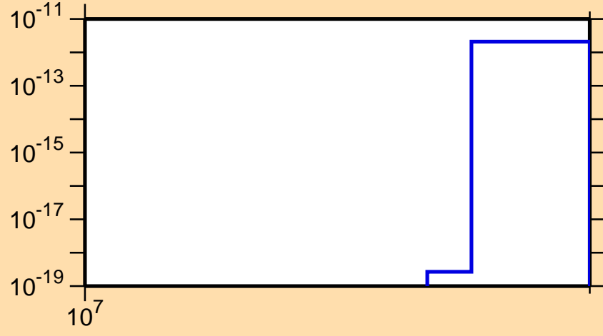
\sigma vs. E for ^{79}\text{Br}(n,pd)
