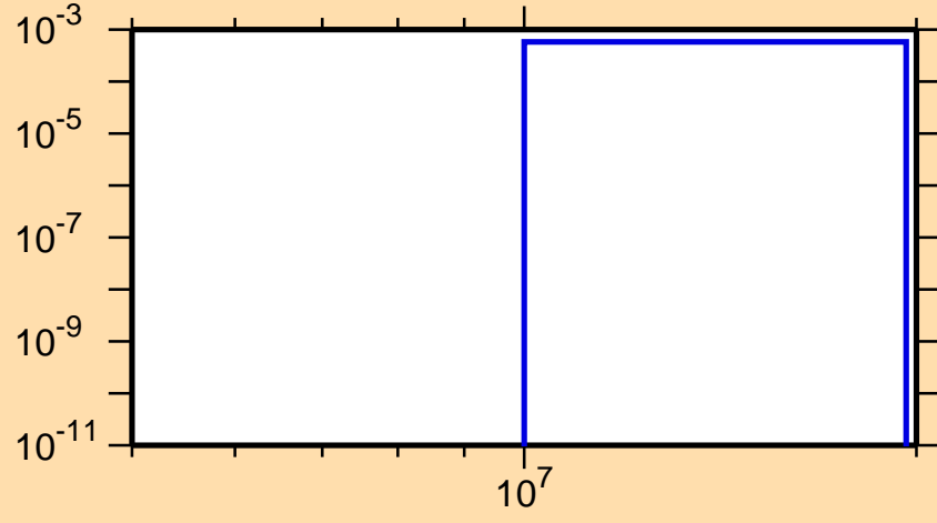
\sigma vs. E for ^{80}\text{Br}(n,\alpha)
