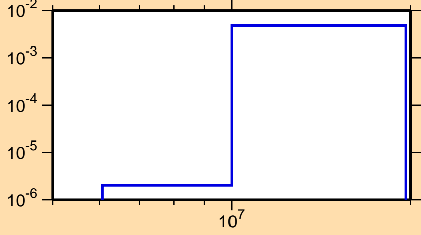
\sigma vs. E for ^{80}\text{Br}(n,d)
