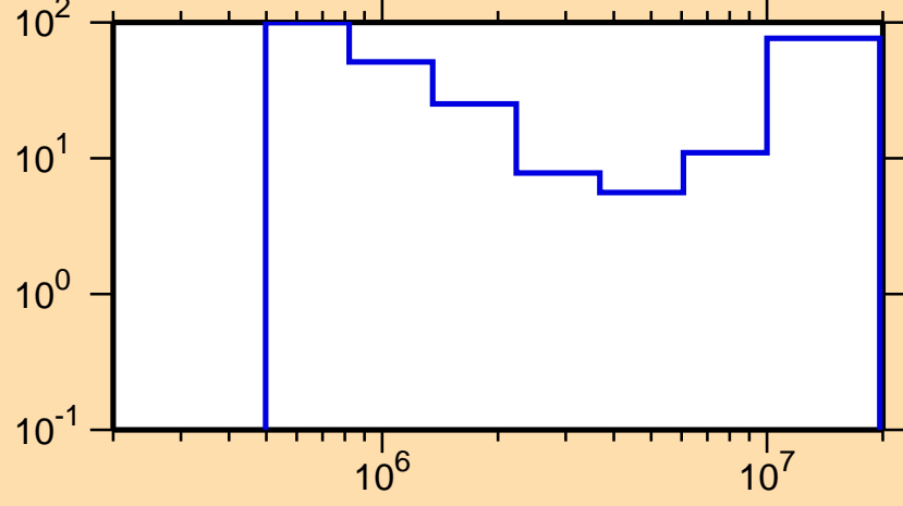
\Delta\sigma/\sigma vs. E for ^{80}\text{Br}(n,ncont.)
