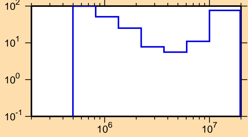
\Delta\sigma/\sigma vs. E for ^{80}\text{Br}(n,n\text{cont.})
