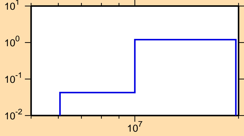
\sigma vs. E for ^{80}\text{Br}(n,2n)
