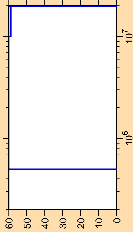
\Delta\sigma/\sigma vs. E for ^{80}\text{Br}(n,p)
