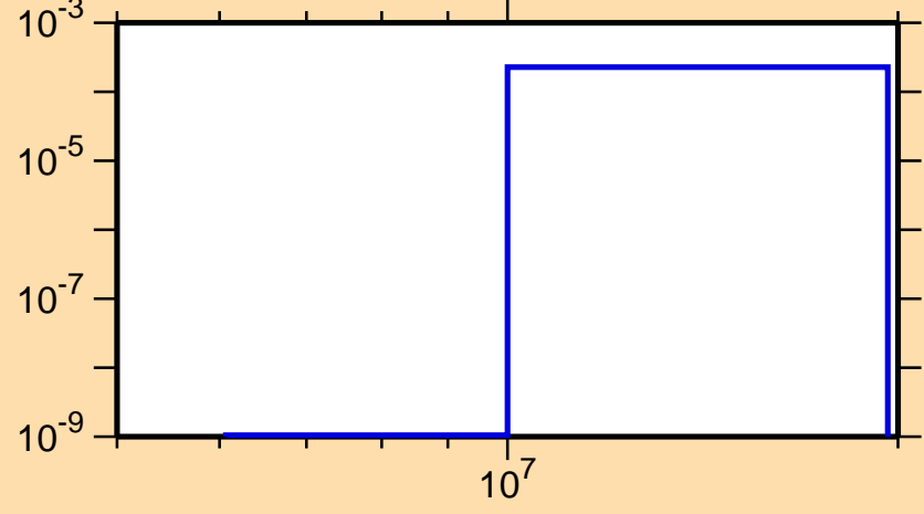
\sigma vs. E for ^{80}\text{Br}(n,t)
