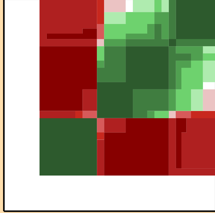
\sigma vs. E for ^{85}\text{Br}(n,n_2)
