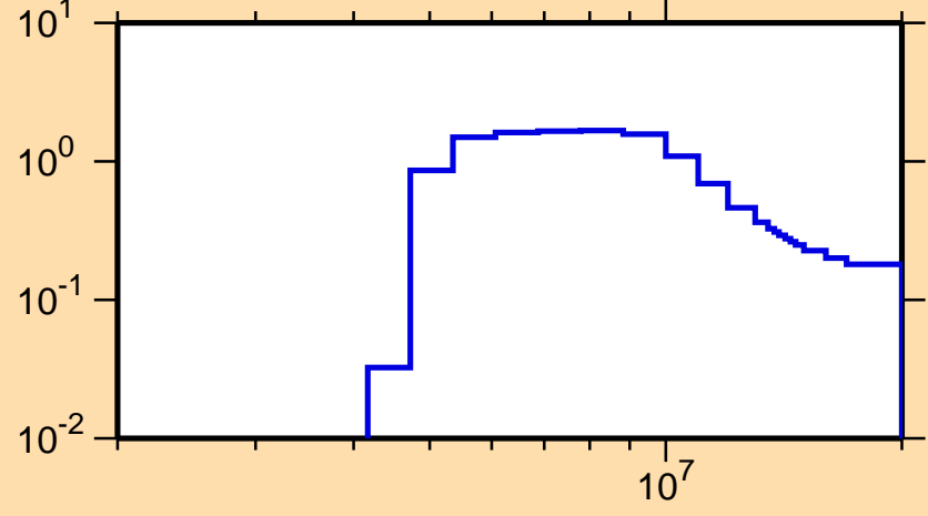
\sigma vs. E for ^{85}\text{Br}(n,n\text{cont.})
