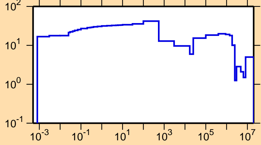
\Delta\sigma/\sigma vs. E for ^{85}\text{Br}(n,\text{tot.})
