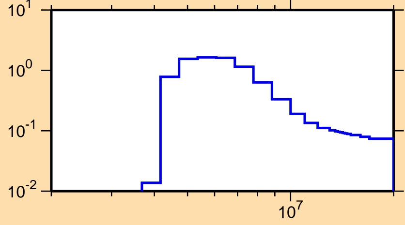
\sigma vs. E for ^{87}\text{Br}(n,n\text{cont.})
