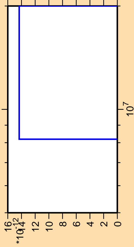
\Delta\sigma/\sigma vs. E for ^{87}\text{Br}(\text{mt } 11)
