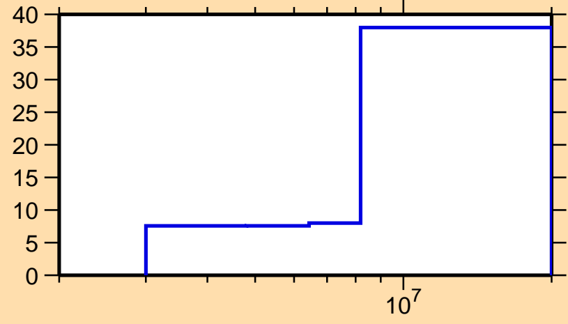
\Delta\sigma/\sigma vs. E for ^{87}\text{Br}(n,inel.)
