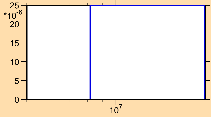
\sigma vs. E for ^{87}\text{Br}(n,t)
