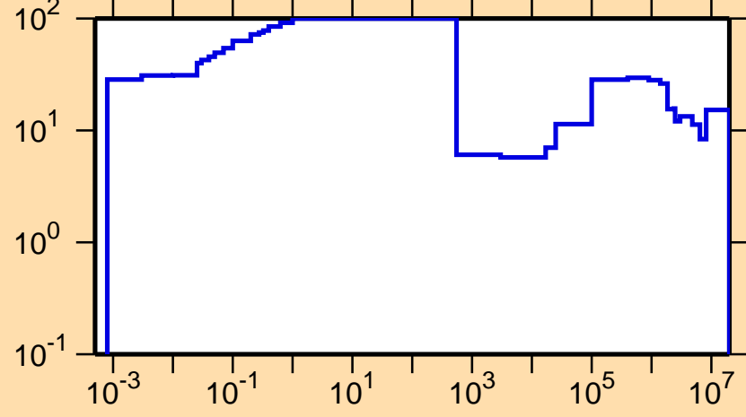
\Delta\sigma/\sigma vs. E for ^{87}\text{Br}(n,\text{tot.})
