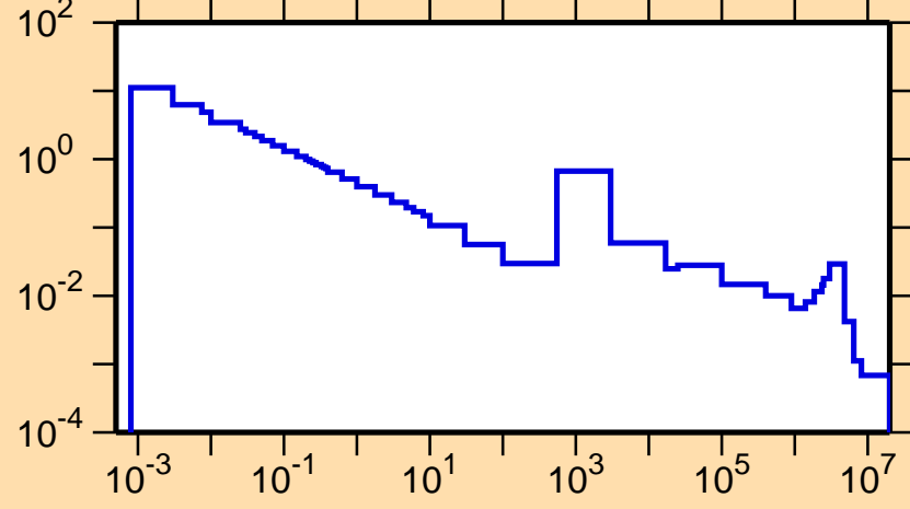
\sigma vs. E for ^{87}\text{Br}(n,\gamma)
