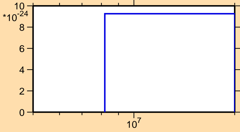
\sigma vs. E for ^{87}\text{Br}(\text{mt } 11)
