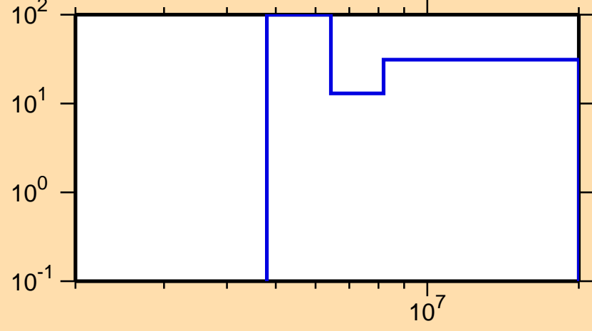
\Delta\sigma/\sigma vs. E for ^{87}\text{Br}(n,2n)
