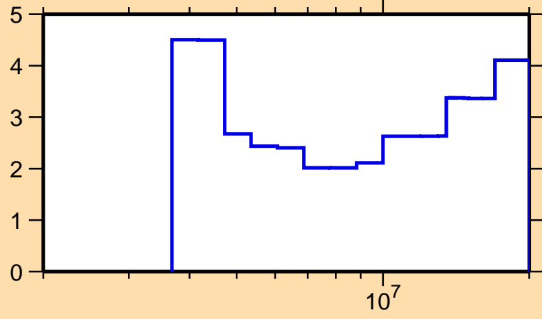
\Delta\sigma/\sigma vs. E for ^{10}\text{C}(n,\text{tot.})
