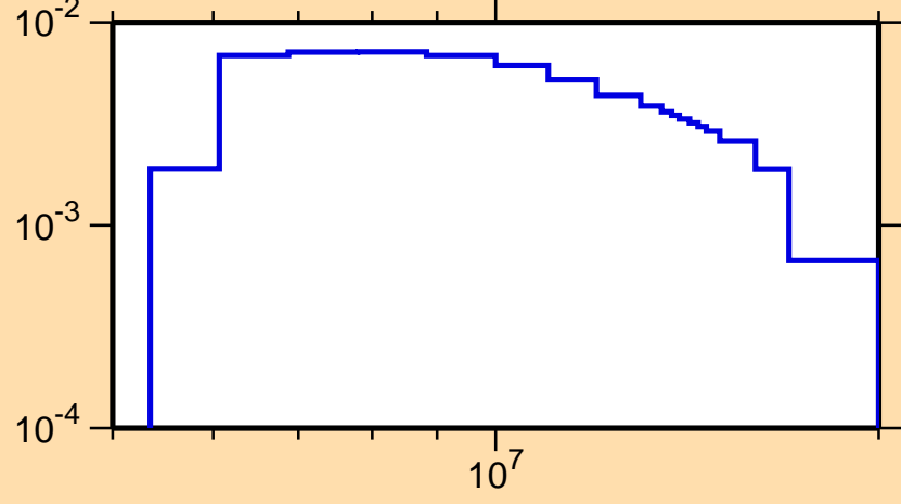
\sigma vs. E for ^{10}\text{C}(n,n_2)
