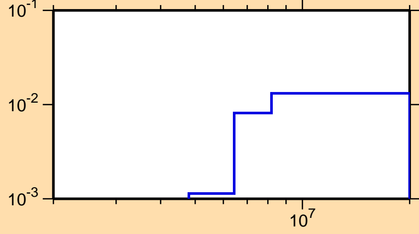
\sigma vs. E for ^{10}\text{C}(n,n\text{cont.})
