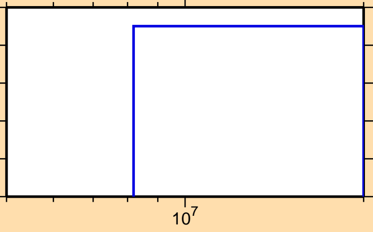
\sigma vs. E for ^{10}\text{C}(n,pt)
