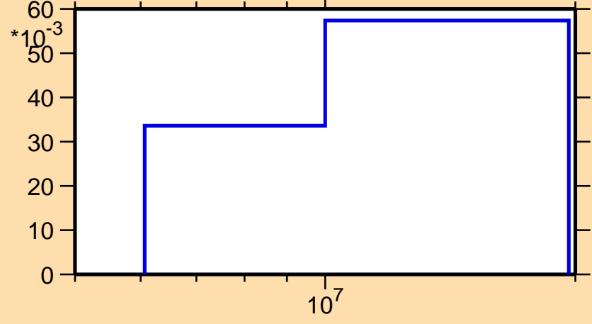
\sigma vs. E for ^{14}\text{C}(n,n_1)
