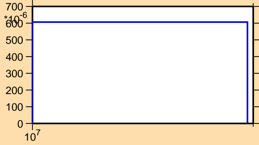
\sigma vs. E for ^{14}\text{C}(n,n\alpha)
