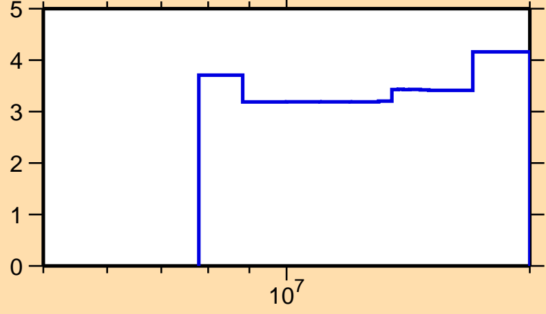
\Delta\sigma/\sigma vs. E for ^{15}\text{C}(n,\text{tot.})
