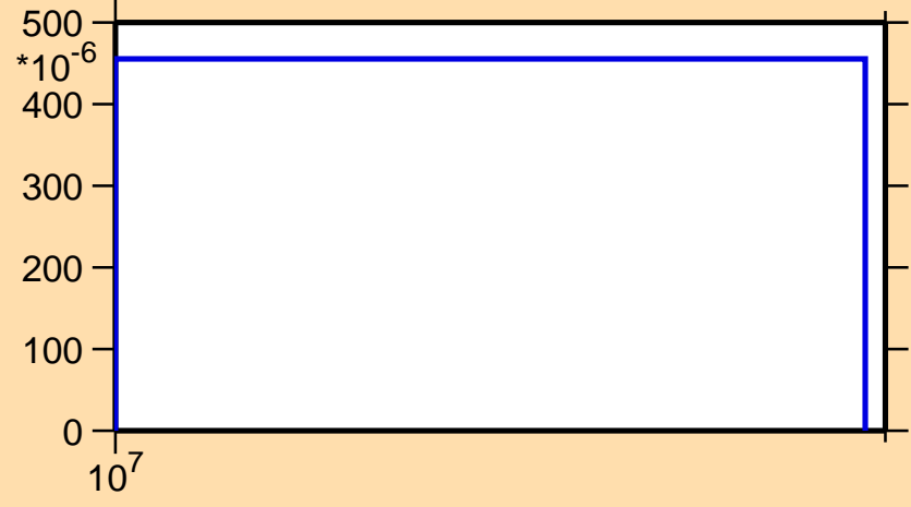
\sigma vs. E for ^{15}\text{C}(n,t)
