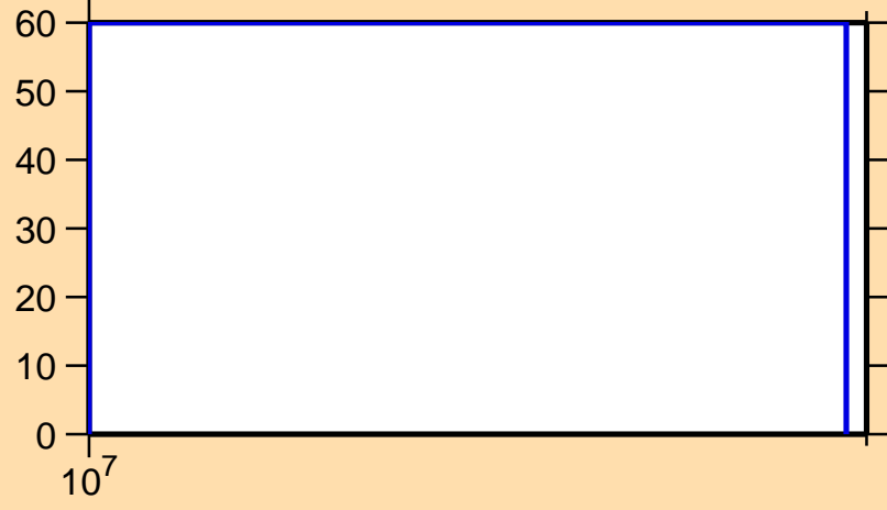
\Delta\sigma/\sigma vs. E for ^{15}\text{C}(n,n\text{cont.})
