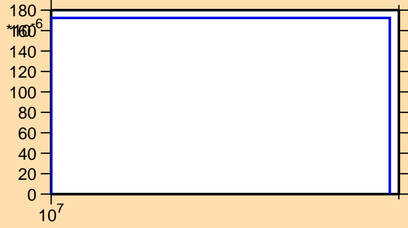
\sigma vs. E for ^{15}\text{C}(n,n\alpha)
