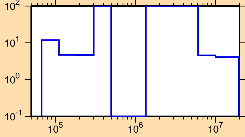
\Delta\sigma/\sigma vs. E for ^{15}\text{C}(n,\text{nonel.})
