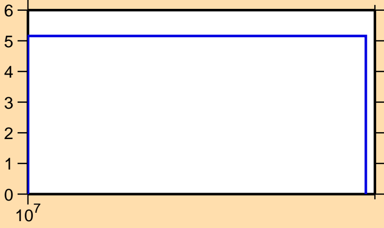
\Delta\sigma/\sigma vs. E for ^{15}\text{C}(n,el.)
