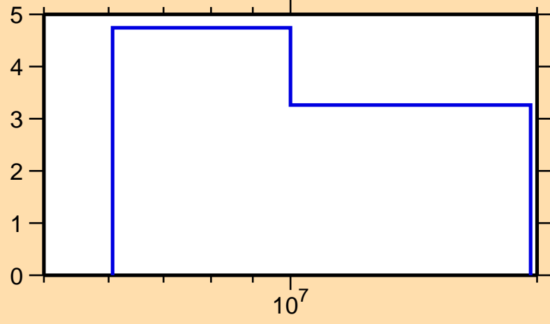
\Delta\sigma/\sigma vs. E for ^{15}\text{C}(n,\text{tot.})
