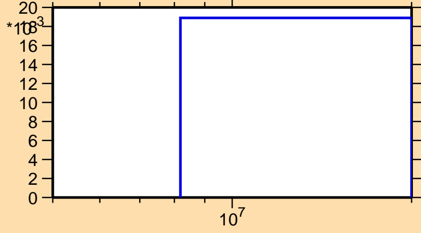
\sigma vs. E for ^{15}\text{C}(n,n_2)
