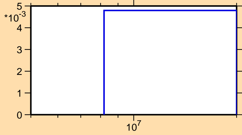
\sigma vs. E for ^{15}\text{C}(n,n\text{cont.})
