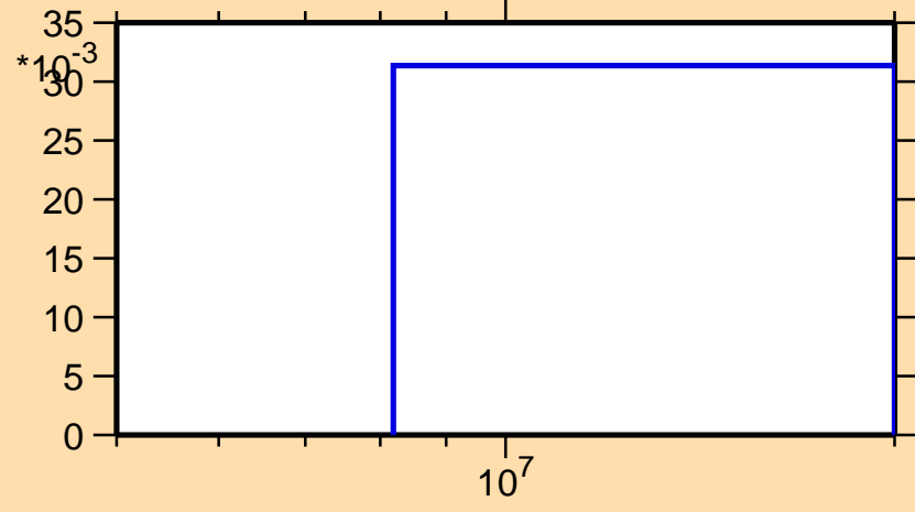
\sigma vs. E for ^{15}\text{C}(n,n_4)
