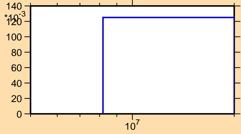
\sigma vs. E for ^{15}\text{C}(n,2n)
