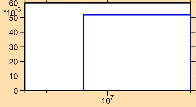
\sigma vs. E for ^{15}\text{C}(n,n_1)
