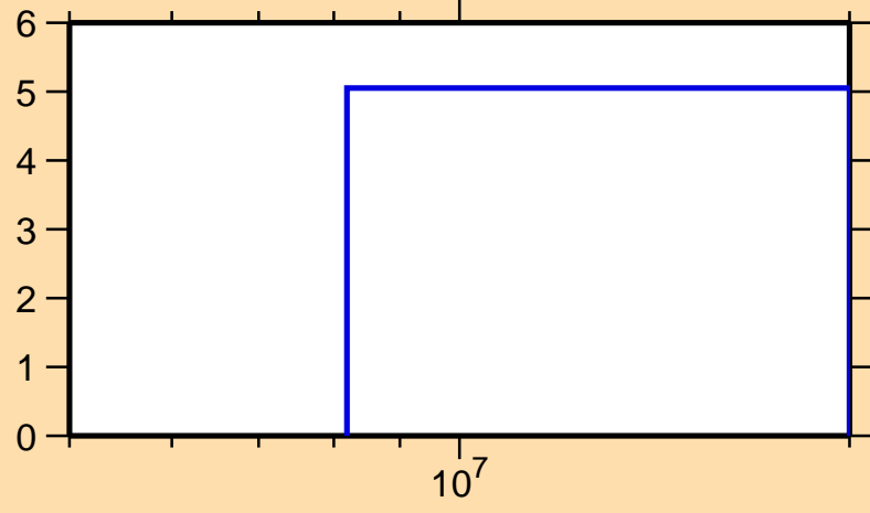
\Delta\sigma/\sigma vs. E for ^{15}\text{C}(n,\text{el.})
