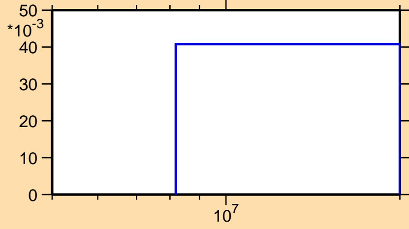
\sigma vs. E for ^{15}\text{C}(n,n_3)
