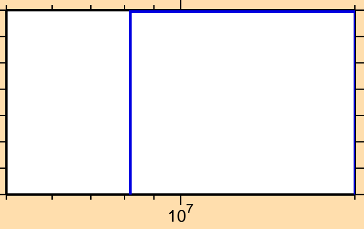
\sigma vs. E for ^{15}\text{C}(n,n\alpha)
