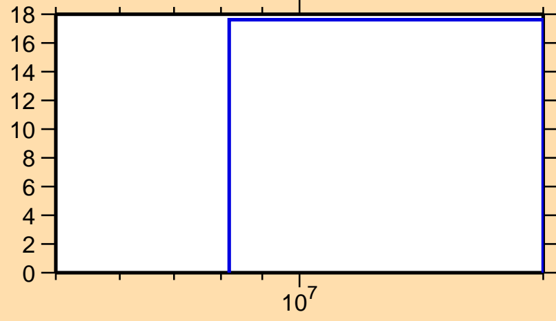
\Delta\sigma/\sigma vs. E for ^{15}\text{C}(n,\text{inel.})
