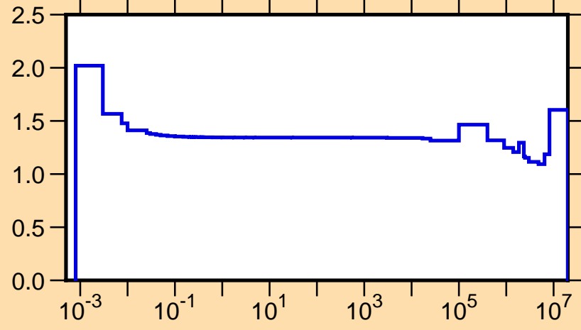
\sigma vs. E for ^{15}\text{C}(n,\text{tot.})
