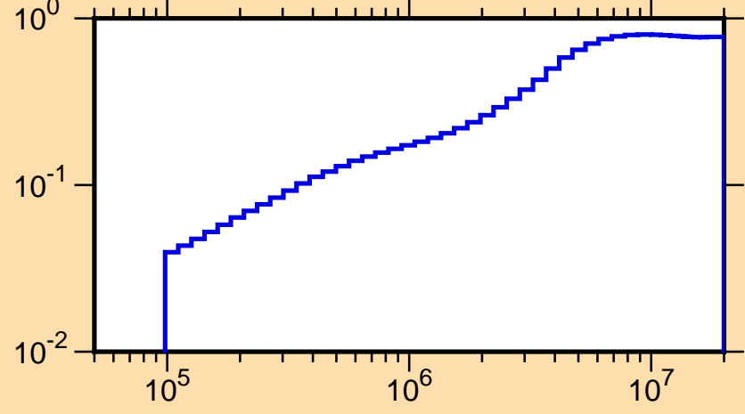
\mu vs. E for ^{40}\text{Ca}(\text{mt251})
