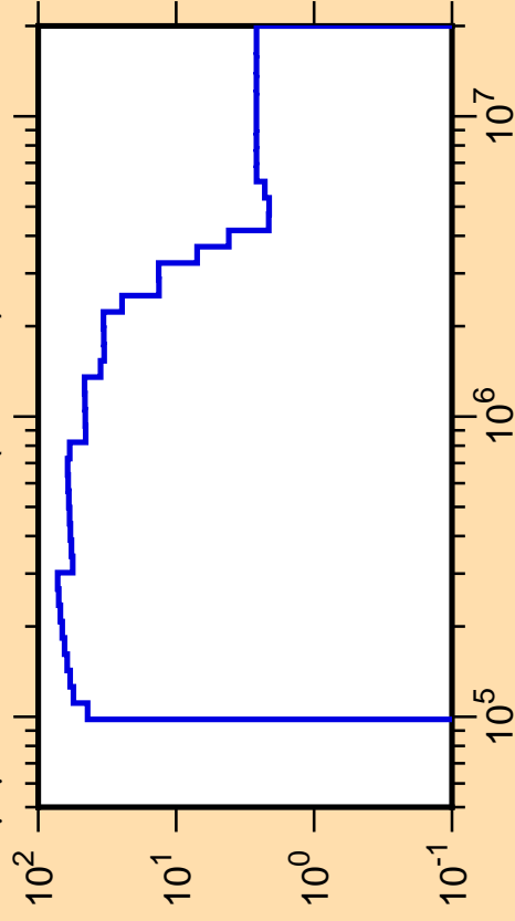
\Delta\mu/\mu vs. E for ^{40}\text{Ca}(\text{mt251})
