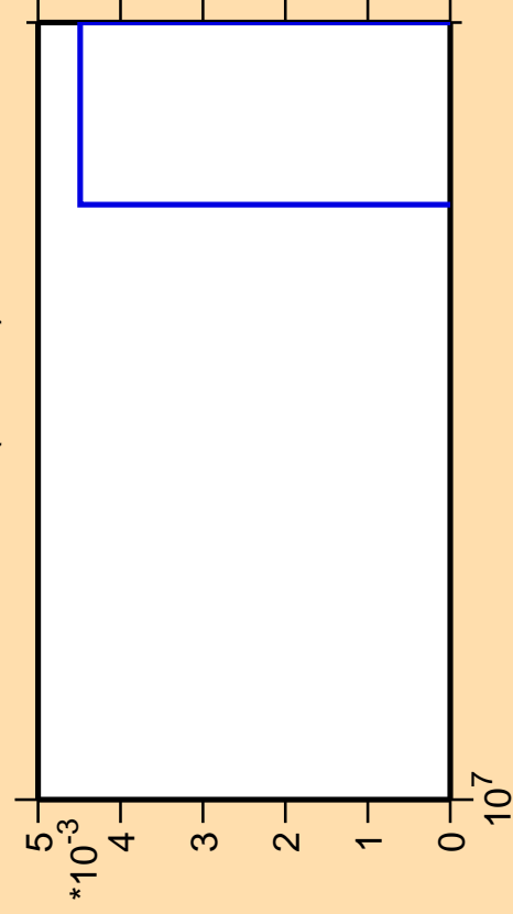
\Delta\sigma/\sigma vs. E for ^{40}\text{Ca} (mt 34)
