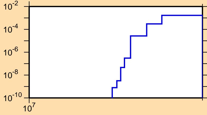
\sigma vs. E for ^{40}\text{Ca}(n,pd)
