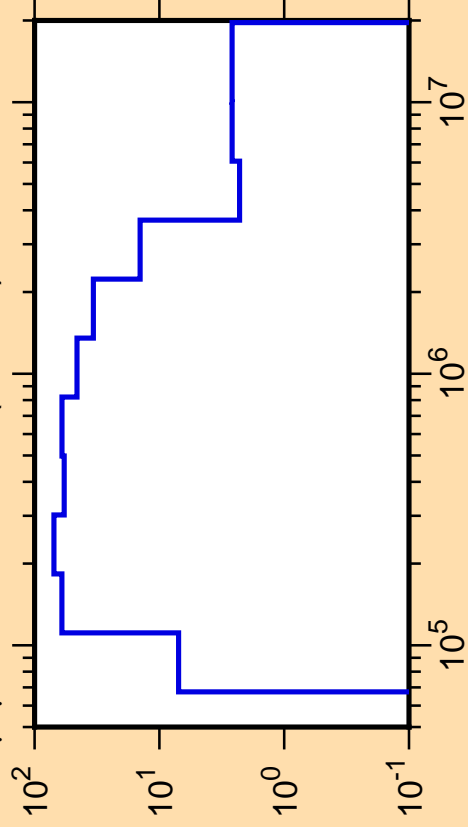
\Delta\mu/\mu vs. E for ^{40}\text{Ca}(\text{mt251})
