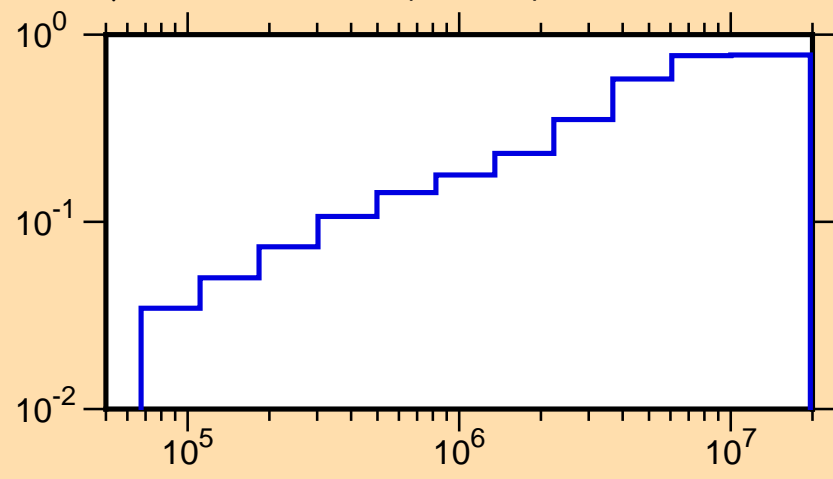
\mu vs. E for ^{40}\text{Ca}(\text{mt251})
