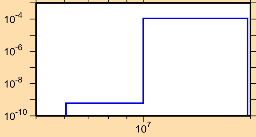
\sigma vs. E for ^{40}\text{Ca}(n,\text{He}3)
