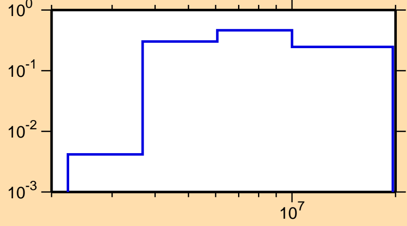
\sigma vs. E for ^{40}\text{Ca}(n,\text{inel.})
