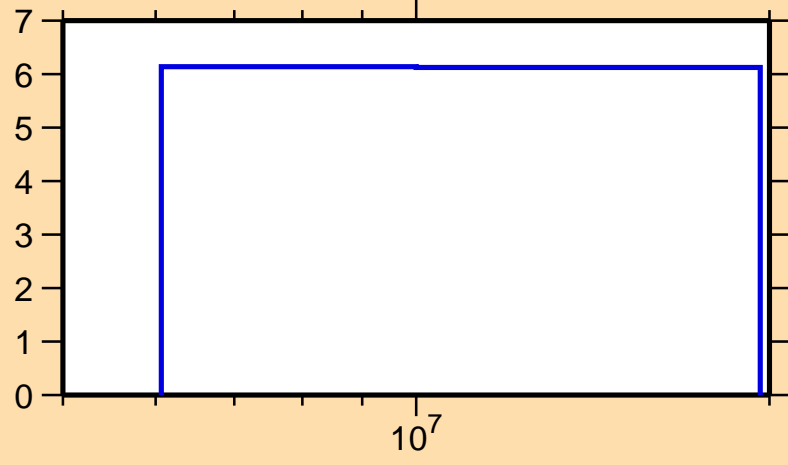
\Delta\sigma/\sigma vs. E for ^{40}\text{Ca}(n,n\text{onel.})
