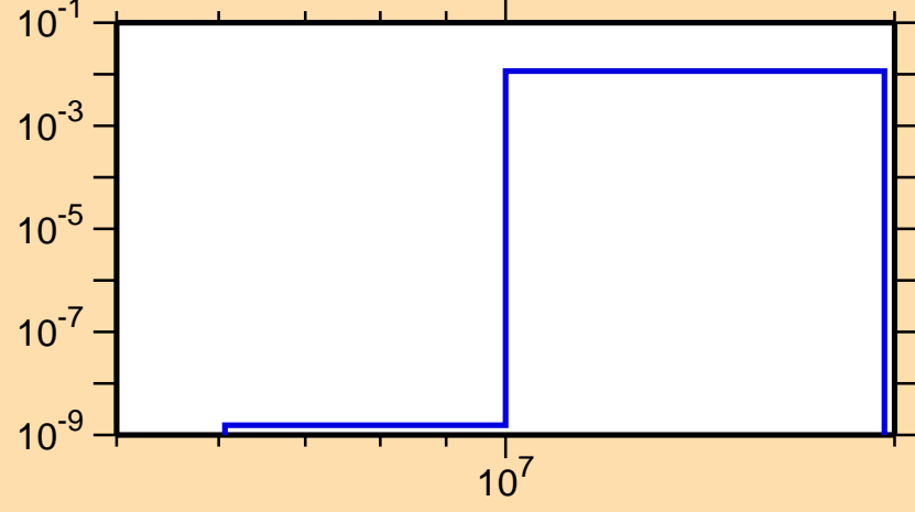
\sigma vs. E for ^{43}\text{Ca}(n,\alpha)
