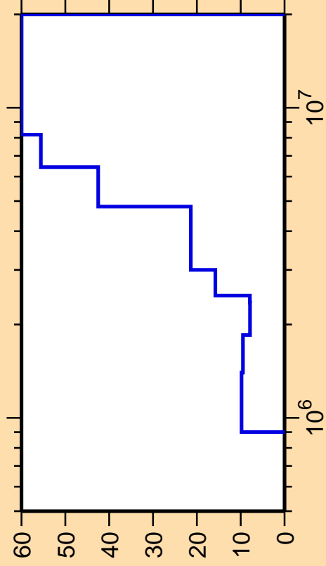
\Delta\sigma/\sigma vs. E for ^{43}\text{Ca}(n,n_3)
