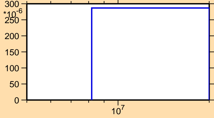
\sigma vs. E for ^{43}\text{Ca}(n,t)
