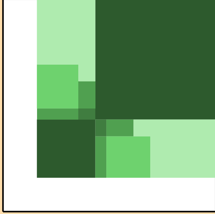
\sigma vs. E for ^{43}\text{Ca}(n,n_3)
