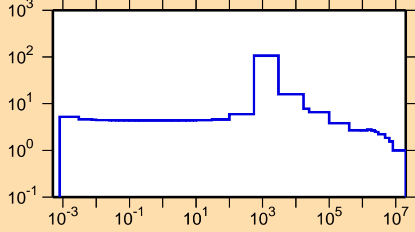
\sigma vs. E for ^{43}\text{Ca}(n,\text{el.})
