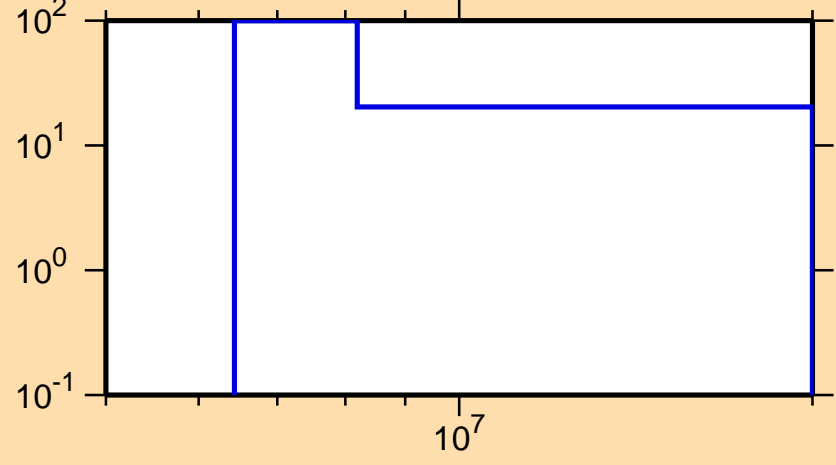
\Delta\sigma/\sigma vs. E for ^{43}\text{Ca}(n,2n)
