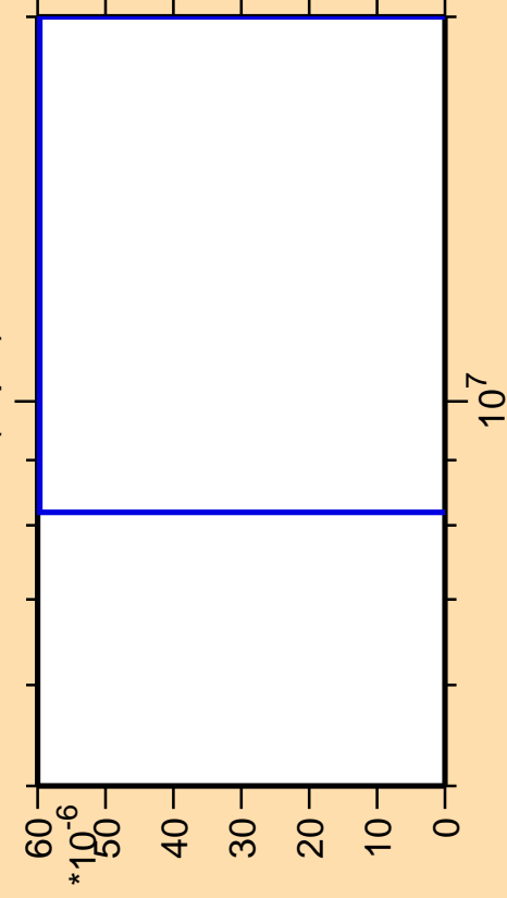
\Delta\sigma/\sigma vs. E for ^{43}\text{Ca}(n,\text{pd})
