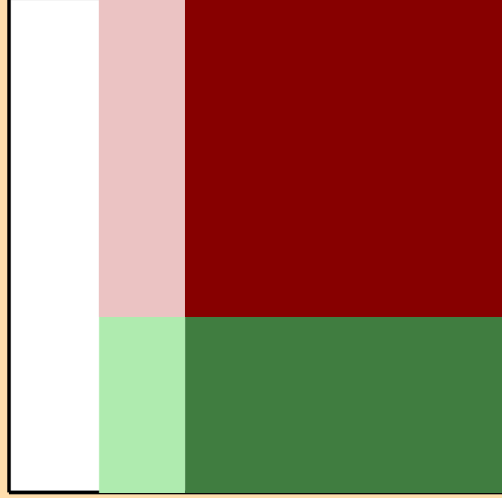
\Delta\sigma/\sigma vs. E for ^{43}\text{Ca}(n,2n)
